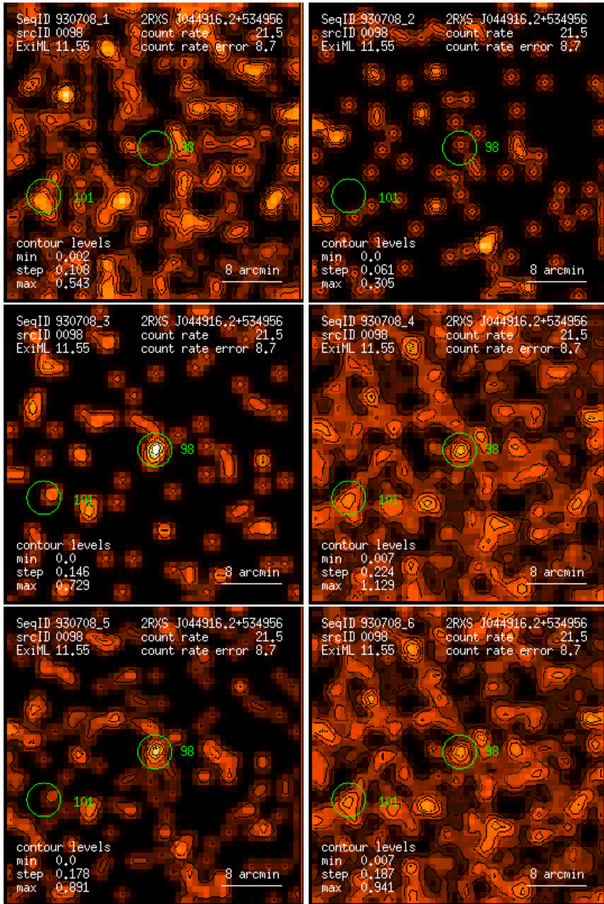
Figure 98: RASS 930708: detection 0098: band rate images, Gaussian filter: (1) PSPC channels 11 – 41, (2) 52 – 90, (3) 91 – 201, (4) 11 – 235, (5) 52 – 201, (6) 11 – 201. Broad band rates in counts/ks. Band rate contour levels in counts/ks/arcmin 2 .
