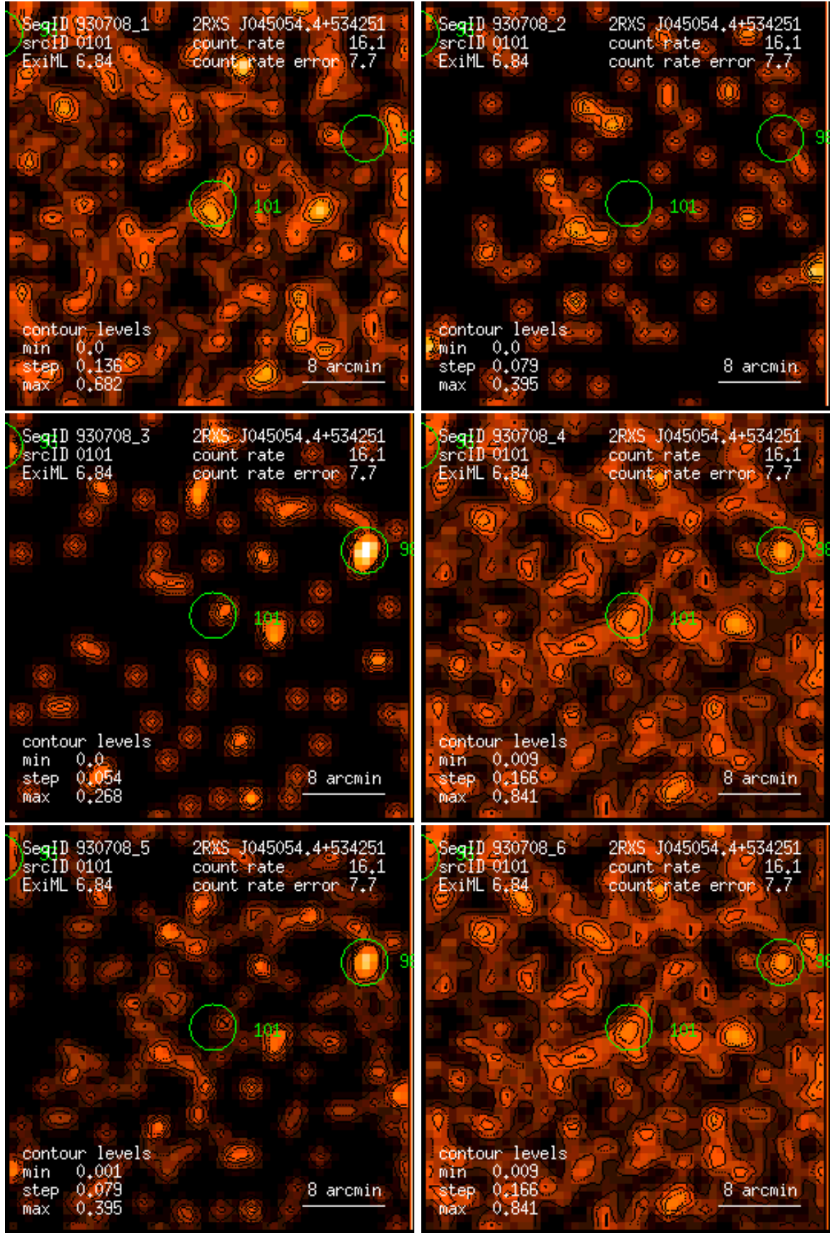
Figure 101: RASS 930708: detection 0101: band rate images, Gaussian filter: (1) PSPC channels 11 – 41, (2) 52 – 90, (3) 91 – 201, (4) 11 – 235, (5) 52 – 201, (6) 11 – 201. Broad band rates in counts/ks. Band rate contour levels in counts/ks/arcmin 2 .
