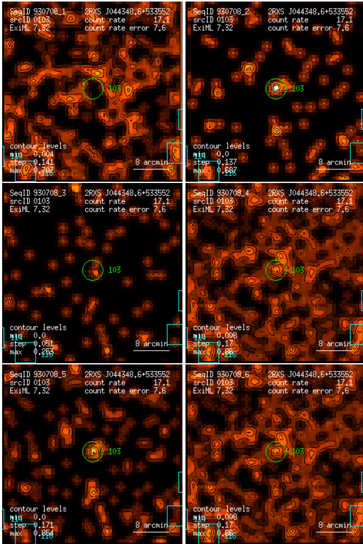
Figure 103: RASS 930708: detection 0103: band rate images, Gaussian filter: (1) PSPC channels 11 – 41, (2) 52 – 90, (3) 91 – 201, (4) 11 – 235, (5) 52 – 201, (6) 11 – 201. Broad band rates in counts/ks. Band rate contour levels in counts/ks/arcmin 2 .
