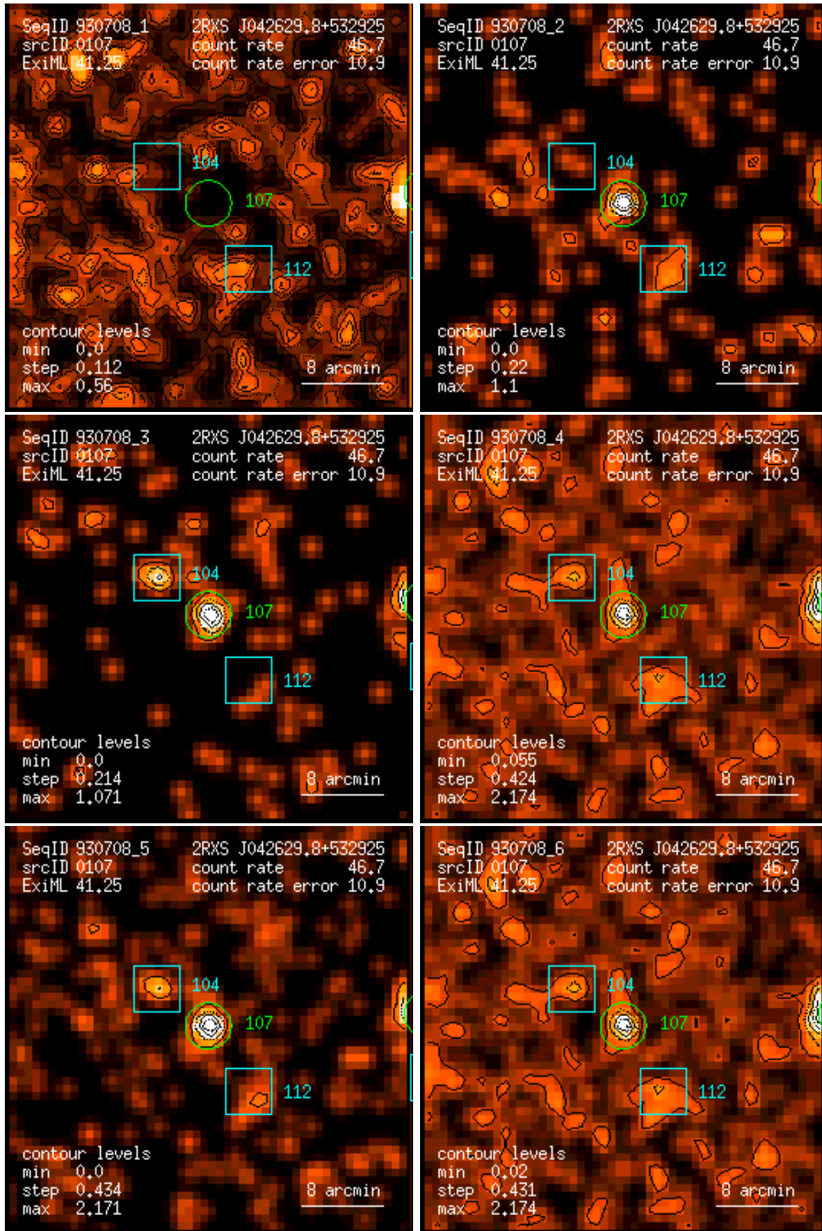
Figure 107: RASS 930708: detection 0107: band rate images, Gaussian filter: (1) PSPC channels 11 – 41, (2) 52 – 90, (3) 91 – 201, (4) 11 – 235, (5) 52 – 201, (6) 11 – 201. Broad band rates in counts/ks. Band rate contour levels in counts/ks/arcmin 2 .
