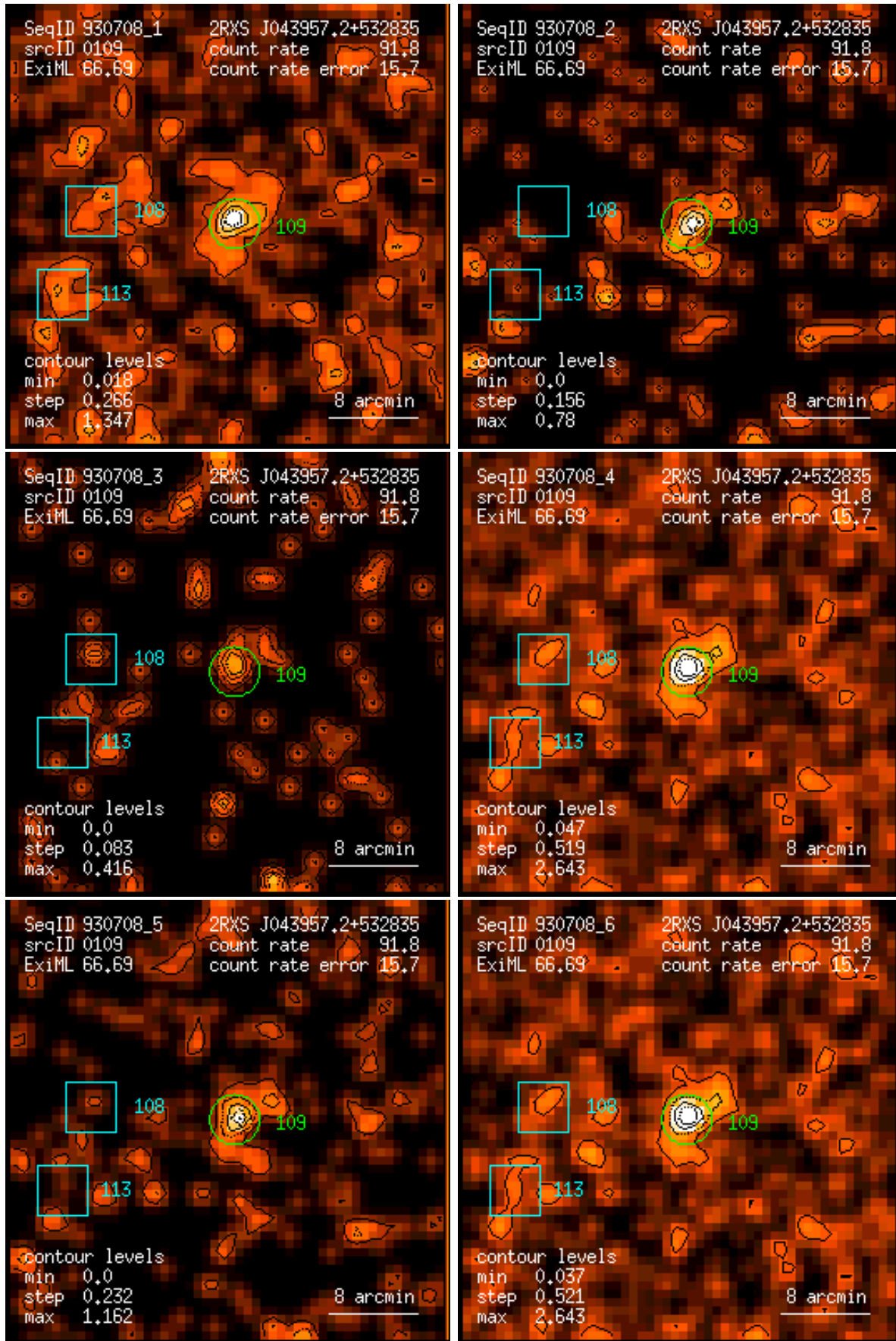
Figure 109: RASS 930708: detection 0109: band rate images, Gaussian filter: (1) PSPC channels 11 – 41, (2) 52 – 90, (3) 91 – 201, (4) 11 – 235, (5) 52 – 201, (6) 11 – 201. Broad band rates in counts/ks. Band rate contour levels in counts/ks/arcmin 2 .
