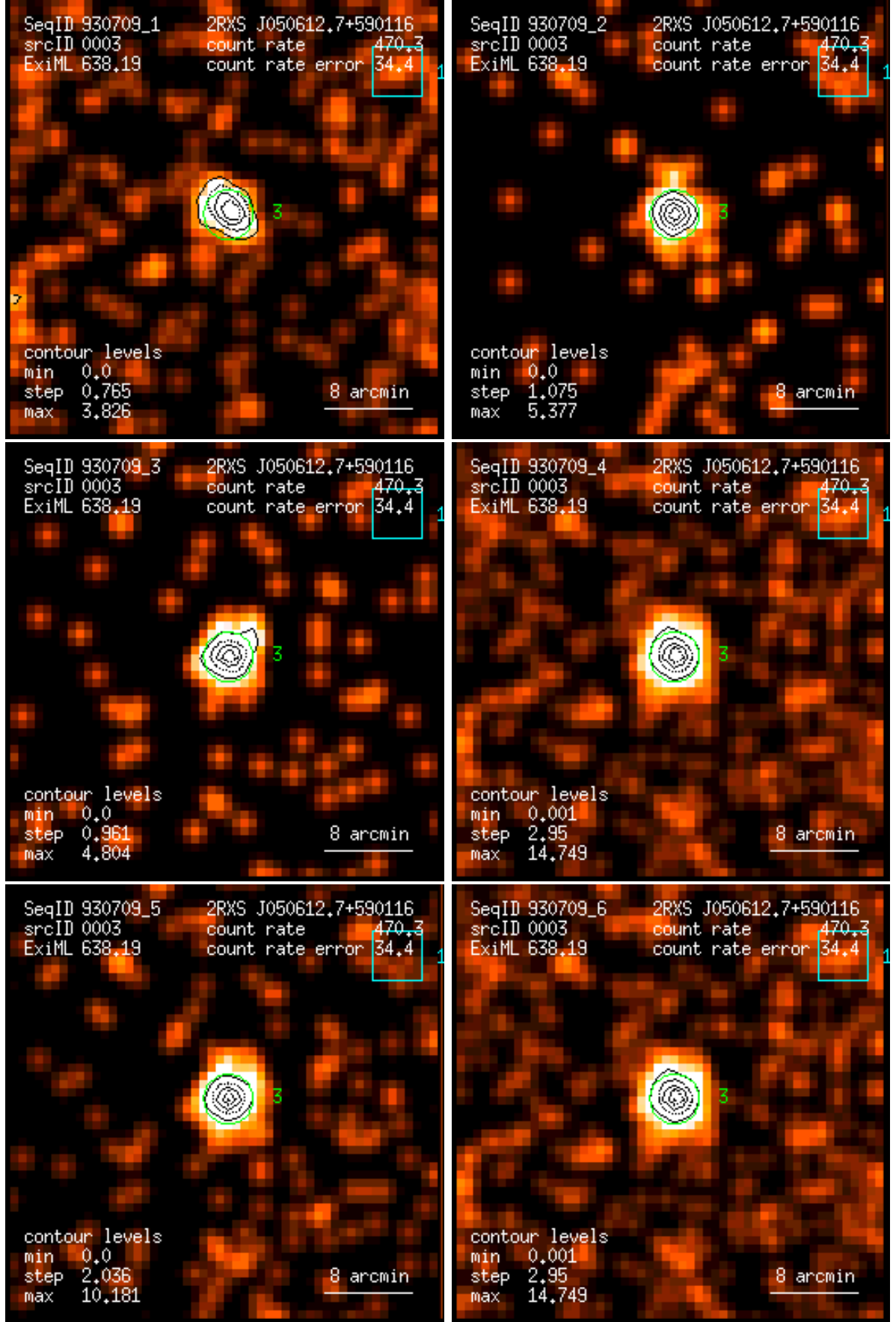
Figure 3: RASS 930709: detection 0003: band rate images, Gaussian filter: (1) PSPC channels 11 – 41, (2) 52 – 90, (3) 91 – 201, (4) 11 – 235, (5) 52 – 201, (6) 11 – 201. Broad band rates in counts/ks. Band rate contour levels in counts/ks/arcmin 2 .
