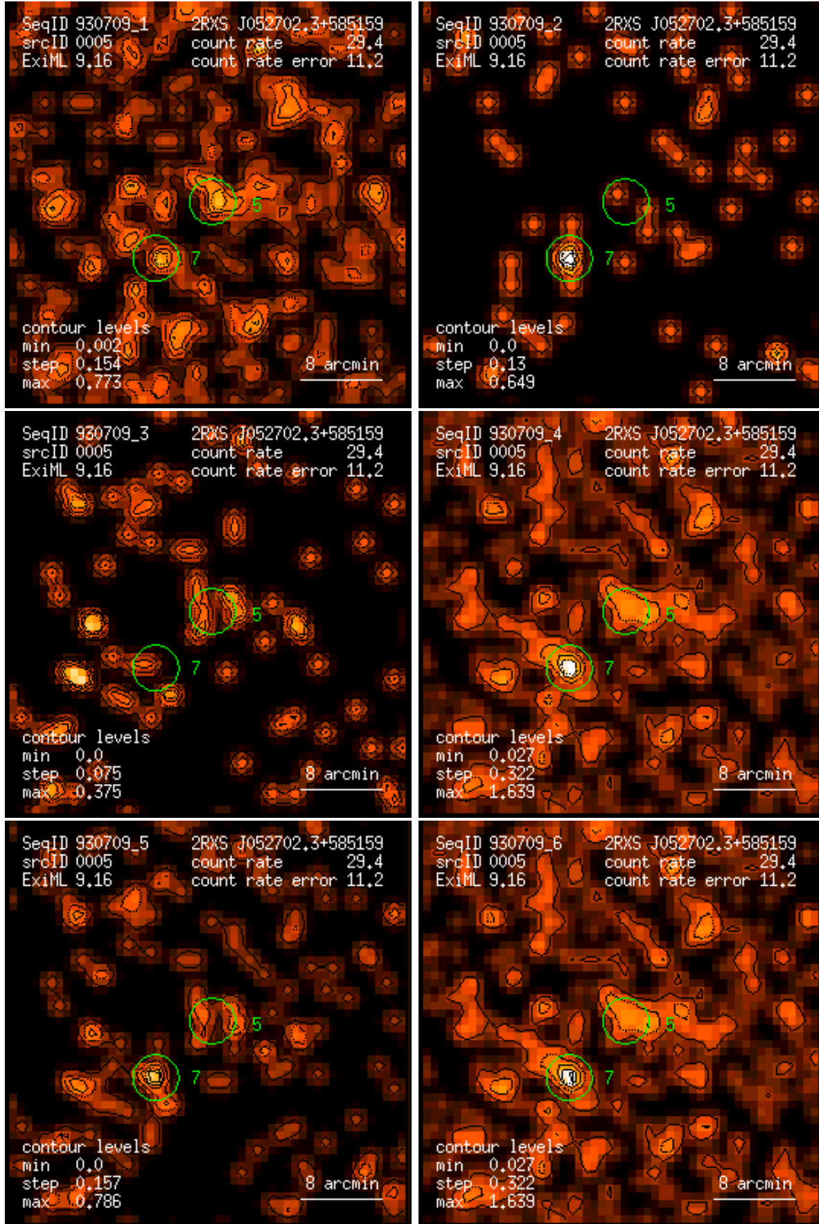
Figure 5: RASS 930709: detection 0005: band rate images, Gaussian filter: (1) PSPC channels 11 – 41, (2) 52 – 90, (3) 91 – 201, (4) 11 – 235, (5) 52 – 201, (6) 11 – 201. Broad band rates in counts/ks. Band rate contour levels in counts/ks/arcmin 2 .
