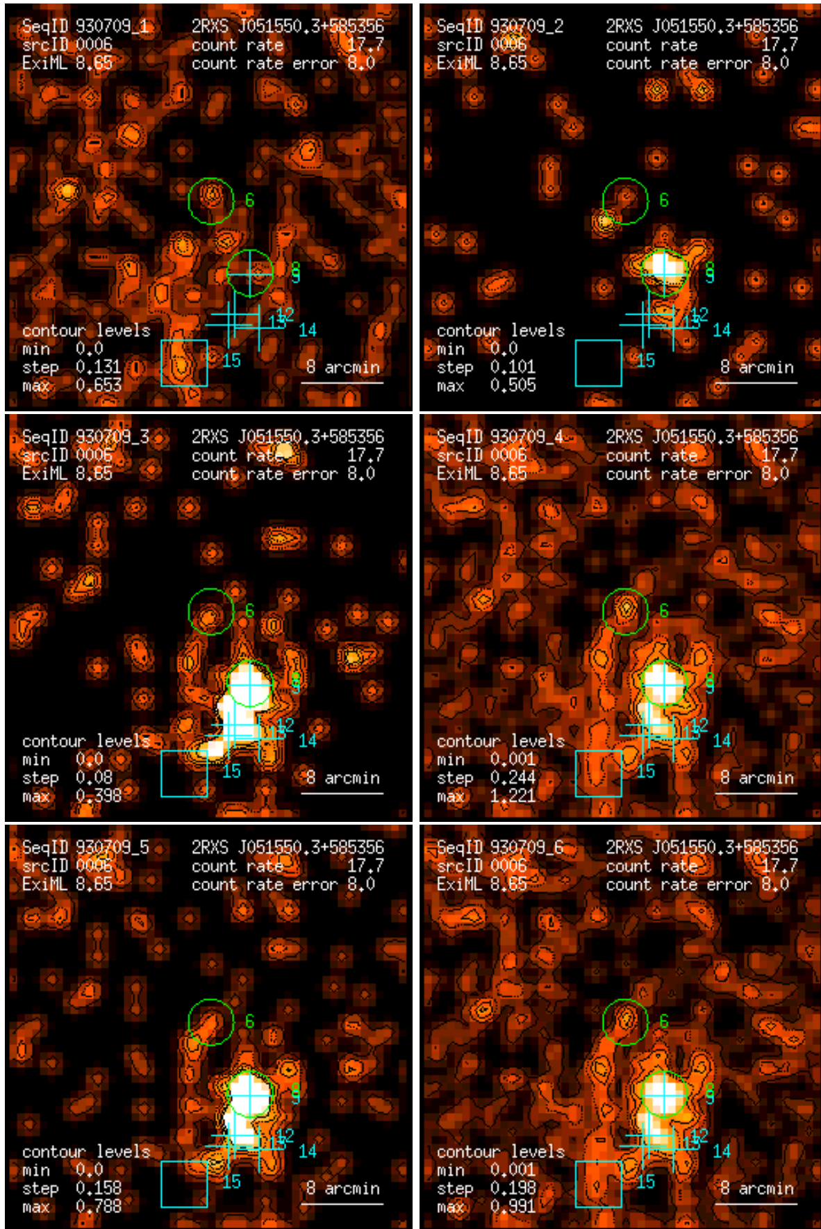
Figure 6: RASS 930709: detection 0006: band rate images, Gaussian filter: (1) PSPC channels 11 – 41, (2) 52 – 90, (3) 91 – 201, (4) 11 – 235, (5) 52 – 201, (6) 11 – 201. Broad band rates in counts/ks. Band rate contour levels in counts/ks/arcmin 2 .
