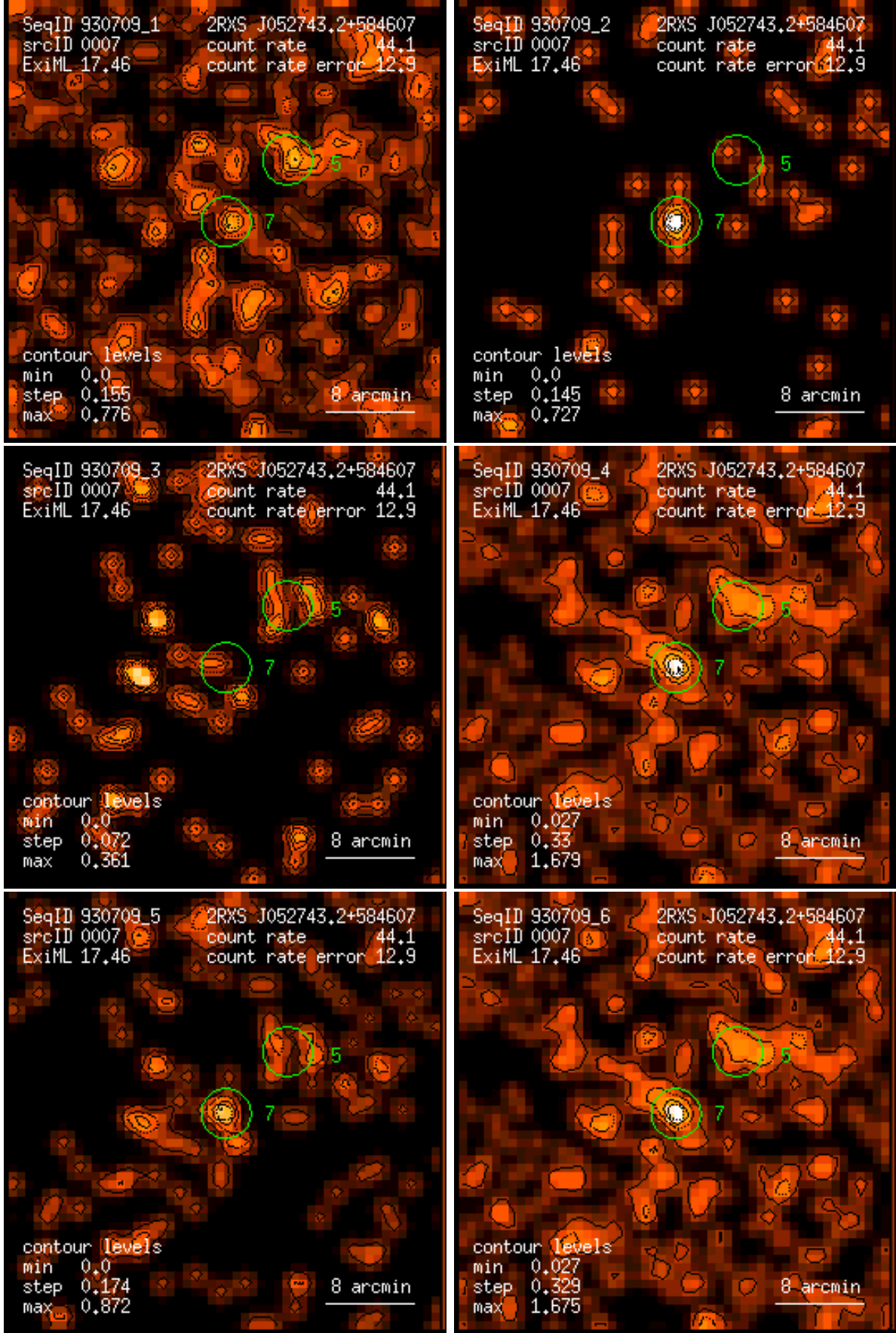
Figure 7: RASS 930709: detection 0007: band rate images, Gaussian filter: (1) PSPC channels 11 – 41, (2) 52 – 90, (3) 91 – 201, (4) 11 – 235, (5) 52 – 201, (6) 11 – 201. Broad band rates in counts/ks. Band rate contour levels in counts/ks/arcmin 2 .
