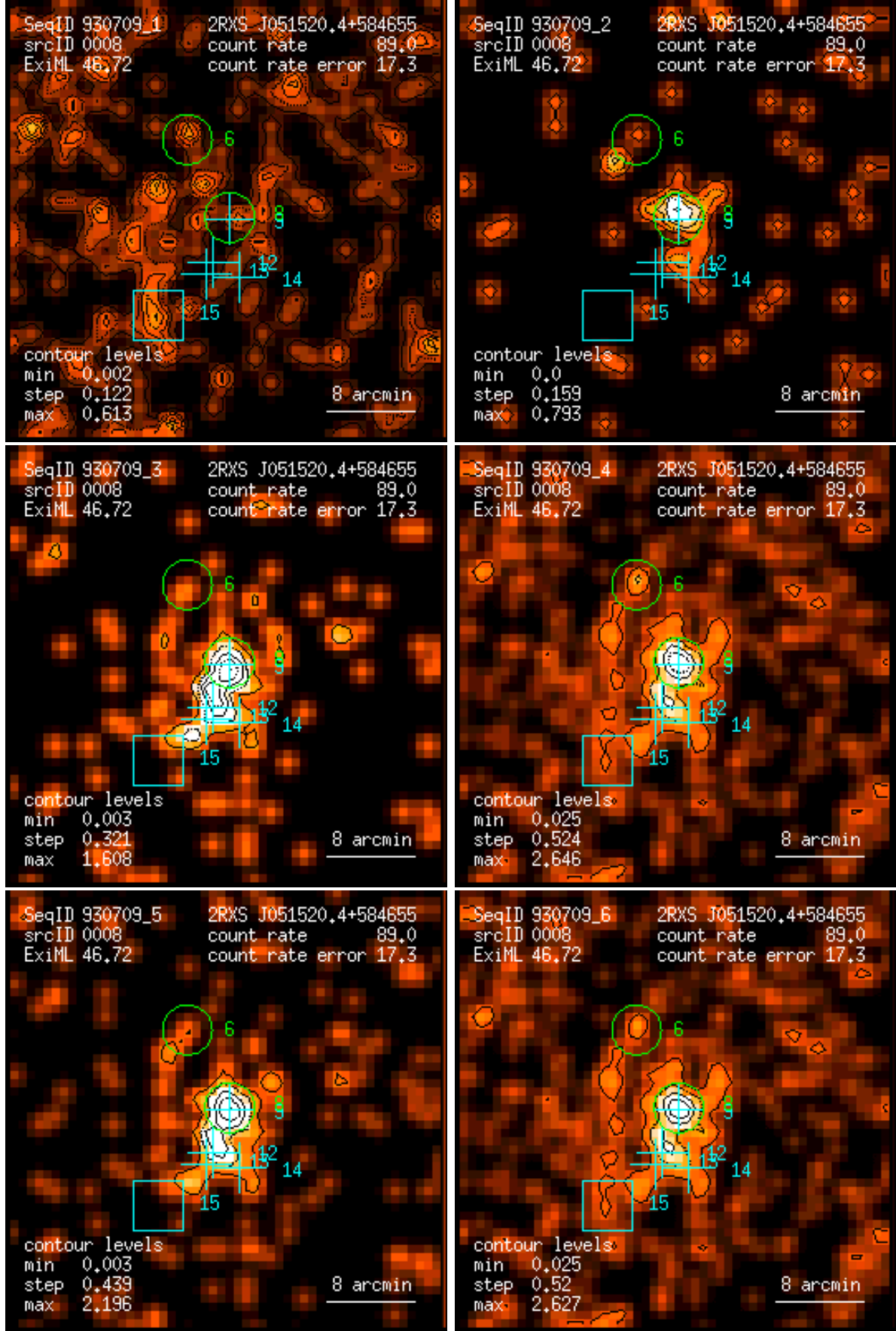
Figure 8: RASS 930709: detection 0008: band rate images, Gaussian filter: (1) PSPC channels 11 – 41, (2) 52 – 90, (3) 91 – 201, (4) 11 – 235, (5) 52 – 201, (6) 11 – 201. Broad band rates in counts/ks. Band rate contour levels in counts/ks/arcmin 2 .
