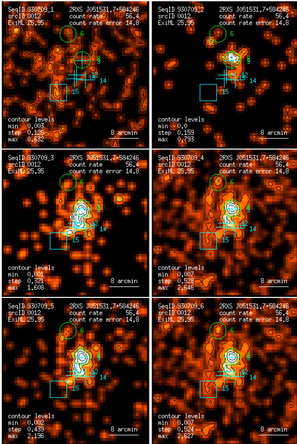
Figure 12: RASS 930709: detection 0012: band rate images, Gaussian filter: (1) PSPC channels 11 – 41, (2) 52 – 90, (3) 91 – 201, (4) 11 – 235, (5) 52 – 201, (6) 11 – 201. Broad band rates in counts/ks. Band rate contour levels in counts/ks/arcmin 2 .
