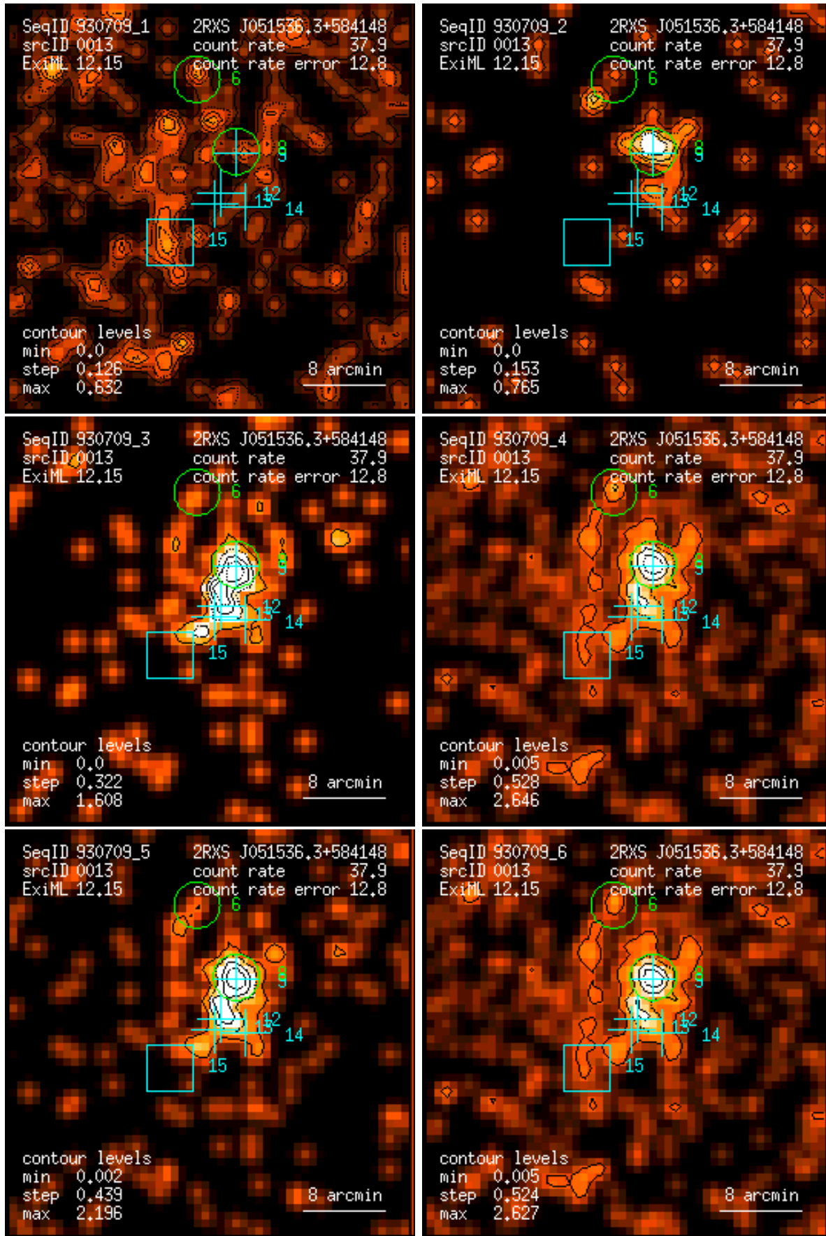
Figure 13: RASS 930709: detection 0013: band rate images, Gaussian filter: (1) PSPC channels 11 – 41, (2) 52 – 90, (3) 91 – 201, (4) 11 – 235, (5) 52 – 201, (6) 11 – 201. Broad band rates in counts/ks. Band rate contour levels in counts/ks/arcmin 2 .
