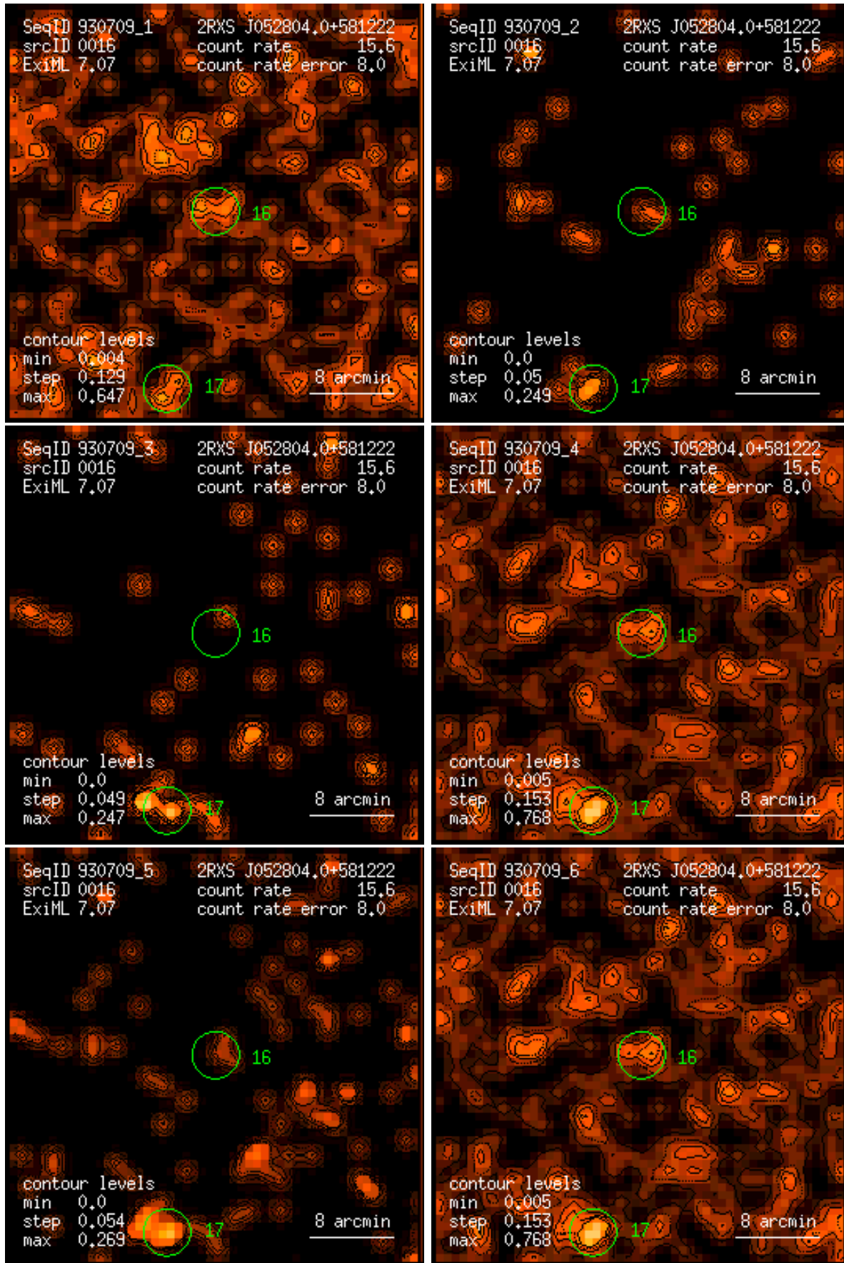
Figure 16: RASS 930709: detection 0016: band rate images, Gaussian filter: (1) PSPC channels 11 – 41, (2) 52 – 90, (3) 91 – 201, (4) 11 – 235, (5) 52 – 201, (6) 11 – 201. Broad band rates in counts/ks. Band rate contour levels in counts/ks/arcmin 2 .
