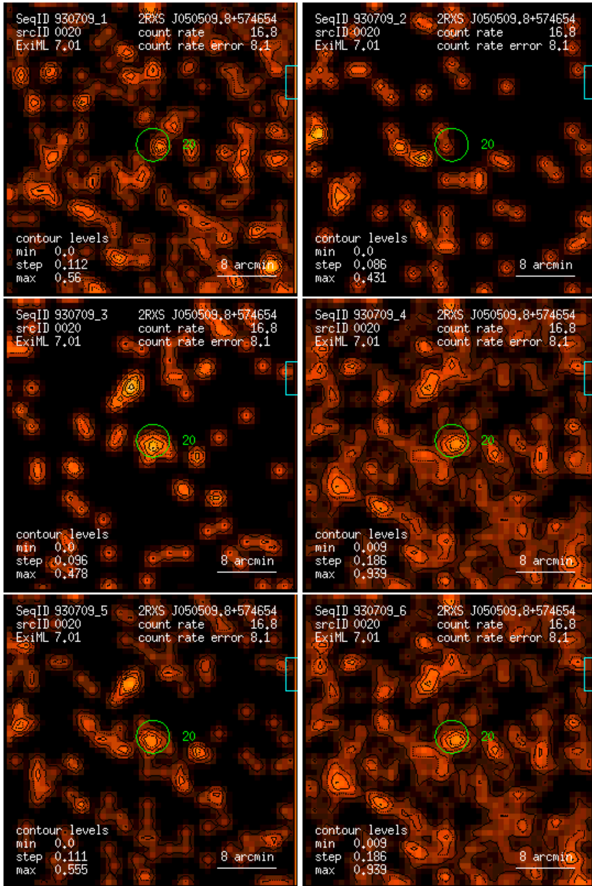
Figure 20: RASS 930709: detection 0020: band rate images, Gaussian filter: (1) PSPC channels 11 – 41, (2) 52 – 90, (3) 91 – 201, (4) 11 – 235, (5) 52 – 201, (6) 11 – 201. Broad band rates in counts/ks. Band rate contour levels in counts/ks/arcmin 2 .
