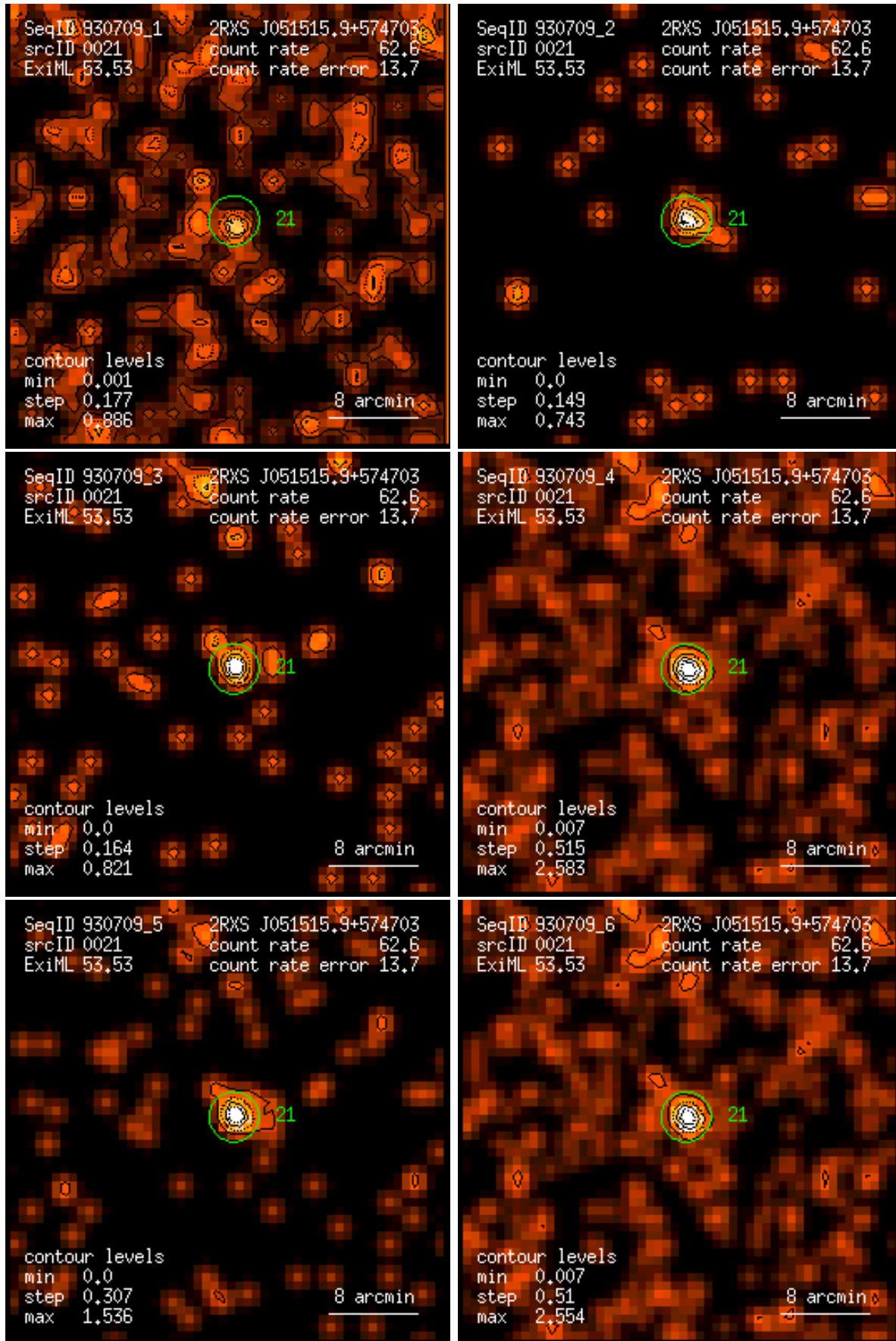
Figure 21: RASS 930709: detection 0021: band rate images, Gaussian filter: (1) PSPC channels 11 – 41, (2) 52 – 90, (3) 91 – 201, (4) 11 – 235, (5) 52 – 201, (6) 11 – 201. Broad band rates in counts/ks. Band rate contour levels in counts/ks/arcmin 2 .
