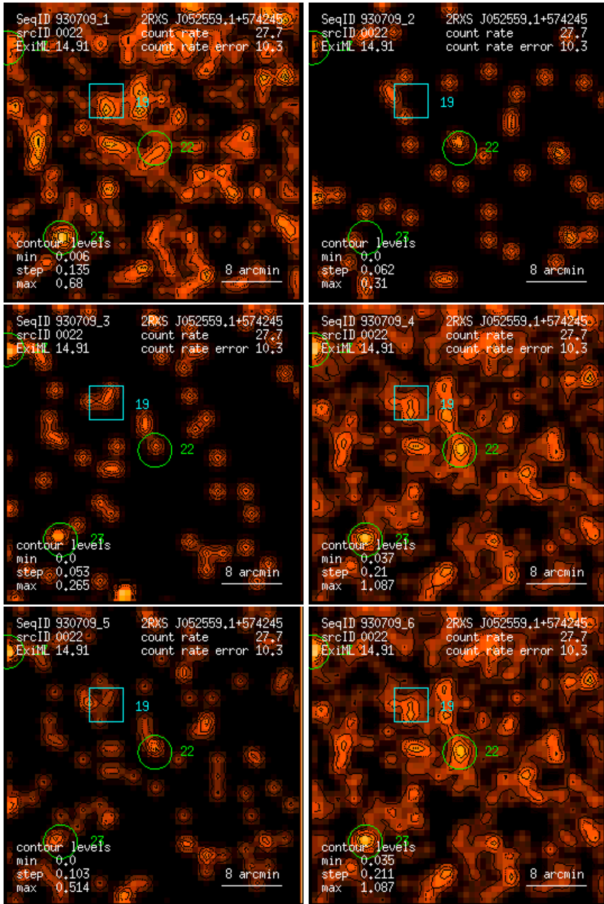
Figure 22: RASS 930709: detection 0022: band rate images, Gaussian filter: (1) PSPC channels 11 – 41, (2) 52 – 90, (3) 91 – 201, (4) 11 – 235, (5) 52 – 201, (6) 11 – 201. Broad band rates in counts/ks. Band rate contour levels in counts/ks/arcmin 2 .
