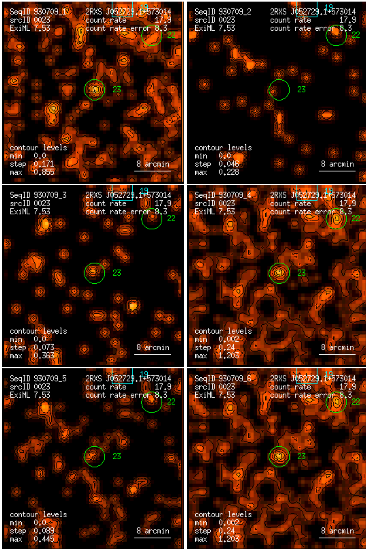
Figure 23: RASS 930709: detection 0023: band rate images, Gaussian filter: (1) PSPC channels 11 – 41, (2) 52 – 90, (3) 91 – 201, (4) 11 – 235, (5) 52 – 201, (6) 11 – 201. Broad band rates in counts/ks. Band rate contour levels in counts/ks/arcmin 2 .
