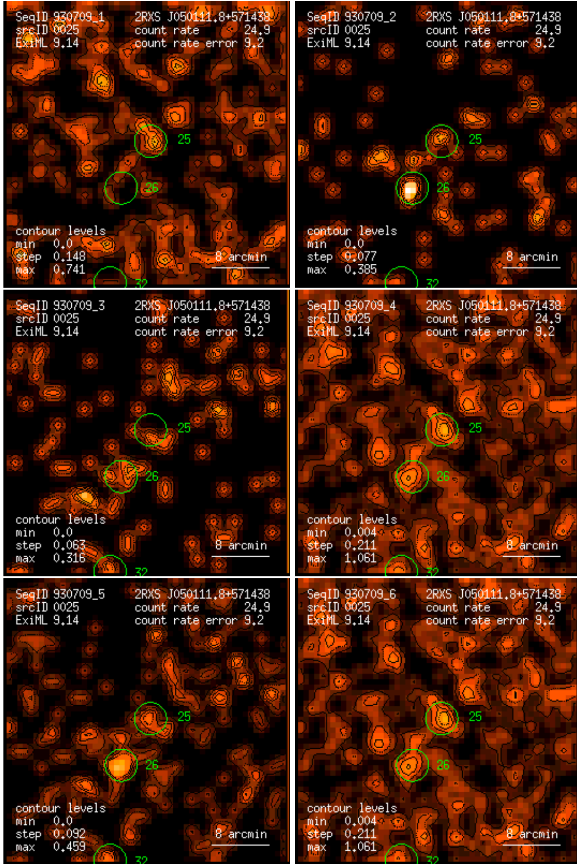
Figure 25: RASS 930709: detection 0025: band rate images, Gaussian filter: (1) PSPC channels 11 – 41, (2) 52 – 90, (3) 91 – 201, (4) 11 – 235, (5) 52 – 201, (6) 11 – 201. Broad band rates in counts/ks. Band rate contour levels in counts/ks/arcmin 2 .
