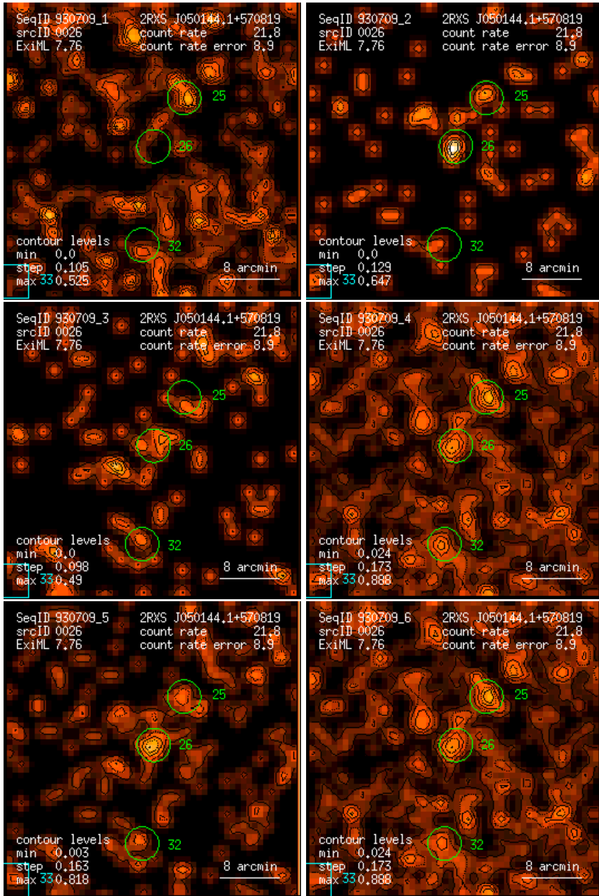
Figure 26: RASS 930709: detection 0026: band rate images, Gaussian filter: (1) PSPC channels 11 – 41, (2) 52 – 90, (3) 91 – 201, (4) 11 – 235, (5) 52 – 201, (6) 11 – 201. Broad band rates in counts/ks. Band rate contour levels in counts/ks/arcmin 2 .
