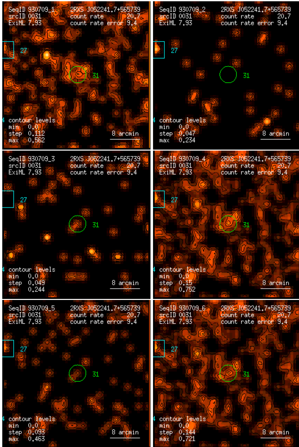
Figure 31: RASS 930709: detection 0031: band rate images, Gaussian filter: (1) PSPC channels 11 – 41, (2) 52 – 90, (3) 91 – 201, (4) 11 – 235, (5) 52 – 201, (6) 11 – 201. Broad band rates in counts/ks. Band rate contour levels in counts/ks/arcmin 2 .
