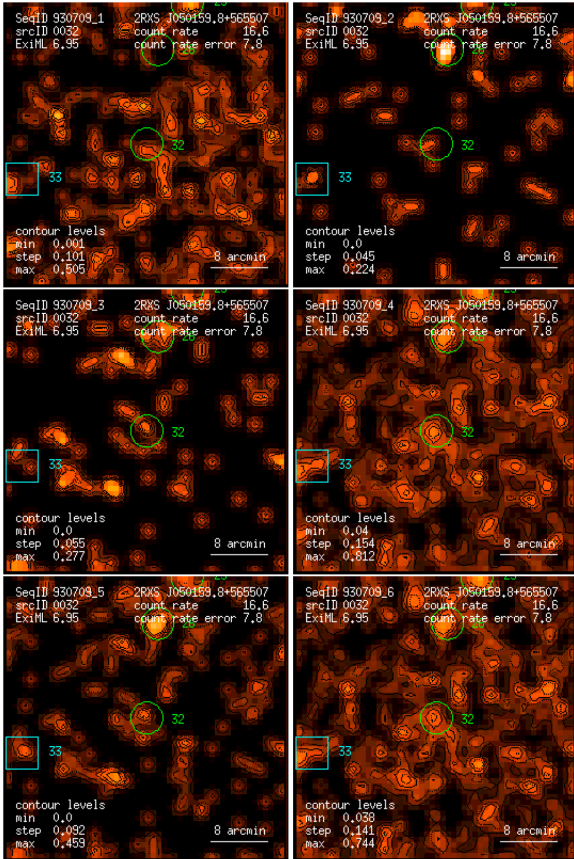
Figure 32: RASS 930709: detection 0032: band rate images, Gaussian filter: (1) PSPC channels 11 – 41, (2) 52 – 90, (3) 91 – 201, (4) 11 – 235, (5) 52 – 201, (6) 11 – 201. Broad band rates in counts/ks. Band rate contour levels in counts/ks/arcmin 2 .
