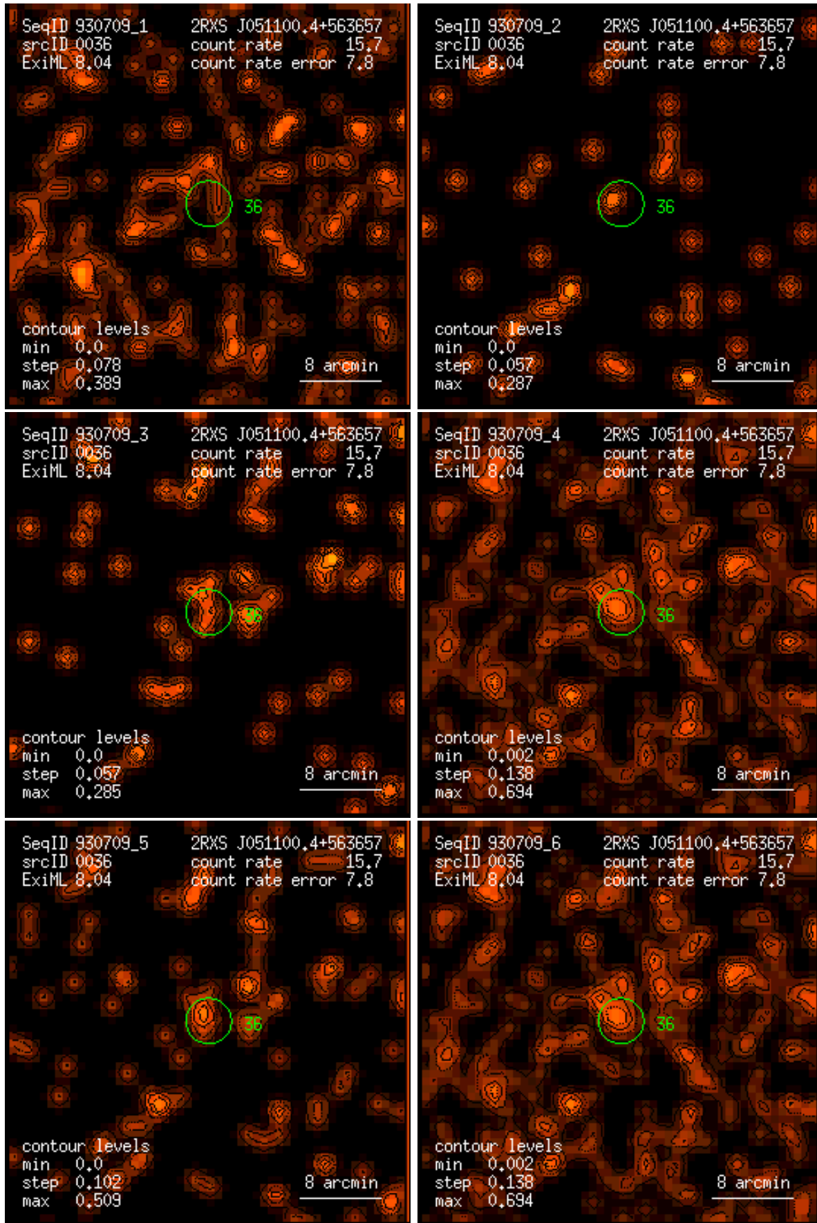
Figure 36: RASS 930709: detection 0036: band rate images, Gaussian filter: (1) PSPC channels 11 – 41, (2) 52 – 90, (3) 91 – 201, (4) 11 – 235, (5) 52 – 201, (6) 11 – 201. Broad band rates in counts/ks. Band rate contour levels in counts/ks/arcmin 2 .
