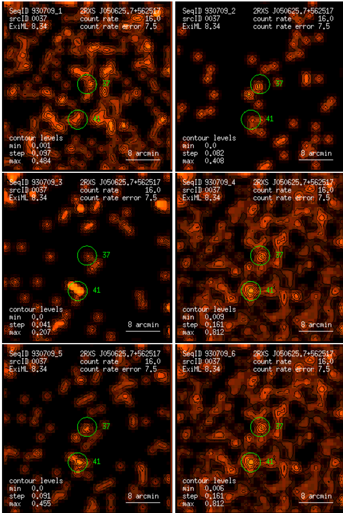
Figure 37: RASS 930709: detection 0037: band rate images, Gaussian filter: (1) PSPC channels 11 – 41, (2) 52 – 90, (3) 91 – 201, (4) 11 – 235, (5) 52 – 201, (6) 11 – 201. Broad band rates in counts/ks. Band rate contour levels in counts/ks/arcmin 2 .
