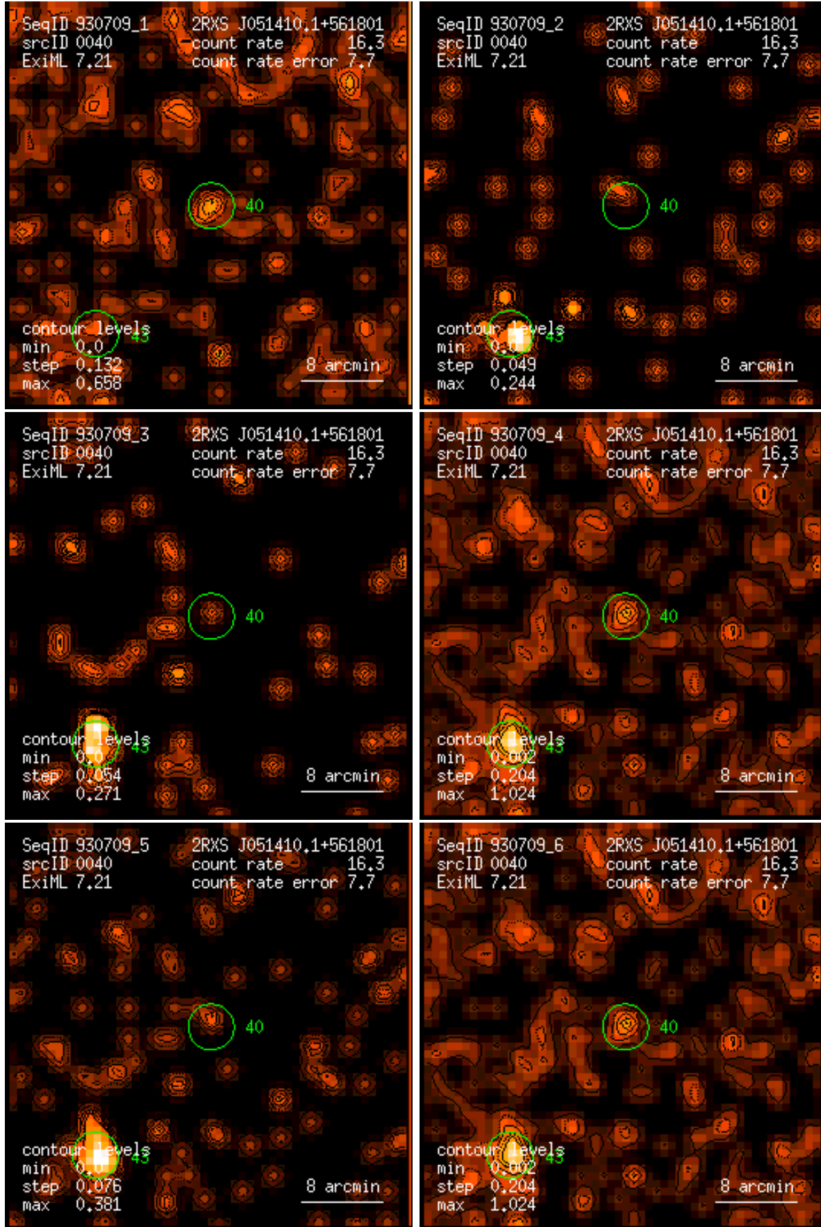
Figure 40: RASS 930709: detection 0040: band rate images, Gaussian filter: (1) PSPC channels 11 – 41, (2) 52 – 90, (3) 91 – 201, (4) 11 – 235, (5) 52 – 201, (6) 11 – 201. Broad band rates in counts/ks. Band rate contour levels in counts/ks/arcmin 2 .
