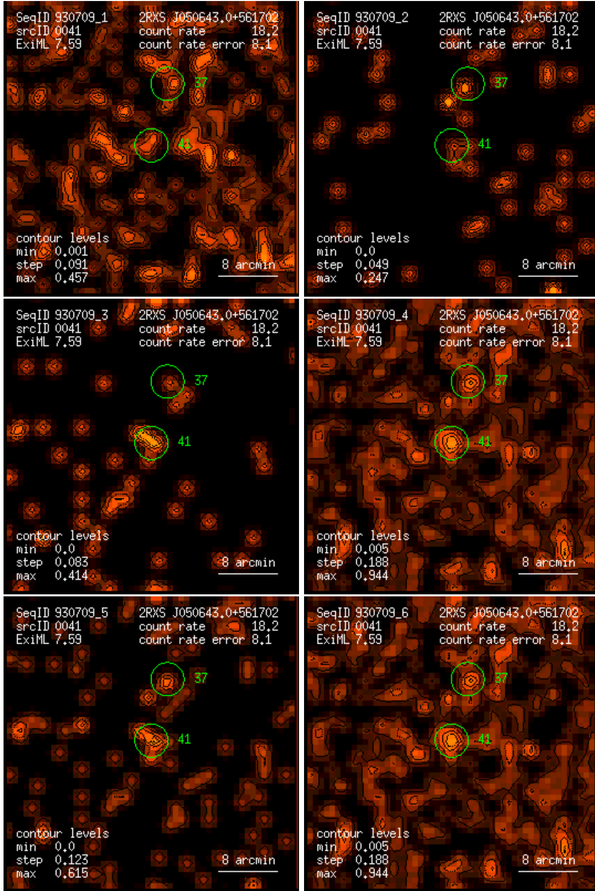
Figure 41: RASS 930709: detection 0041: band rate images, Gaussian filter: (1) PSPC channels 11 – 41, (2) 52 – 90, (3) 91 – 201, (4) 11 – 235, (5) 52 – 201, (6) 11 – 201. Broad band rates in counts/ks. Band rate contour levels in counts/ks/arcmin 2 .
