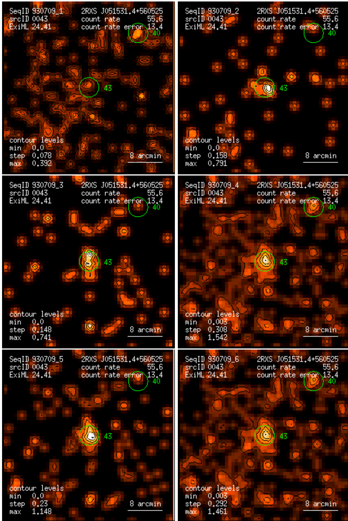
Figure 43: RASS 930709: detection 0043: band rate images, Gaussian filter: (1) PSPC channels 11 – 41, (2) 52 – 90, (3) 91 – 201, (4) 11 – 235, (5) 52 – 201, (6) 11 – 201. Broad band rates in counts/ks. Band rate contour levels in counts/ks/arcmin 2 .
