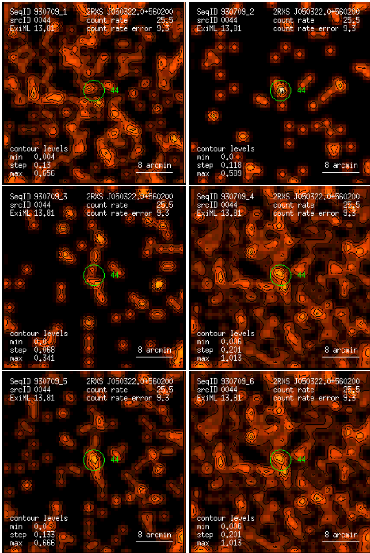
Figure 44: RASS 930709: detection 0044: band rate images, Gaussian filter: (1) PSPC channels 11 – 41, (2) 52 – 90, (3) 91 – 201, (4) 11 – 235, (5) 52 – 201, (6) 11 – 201. Broad band rates in counts/ks. Band rate contour levels in counts/ks/arcmin 2 .
