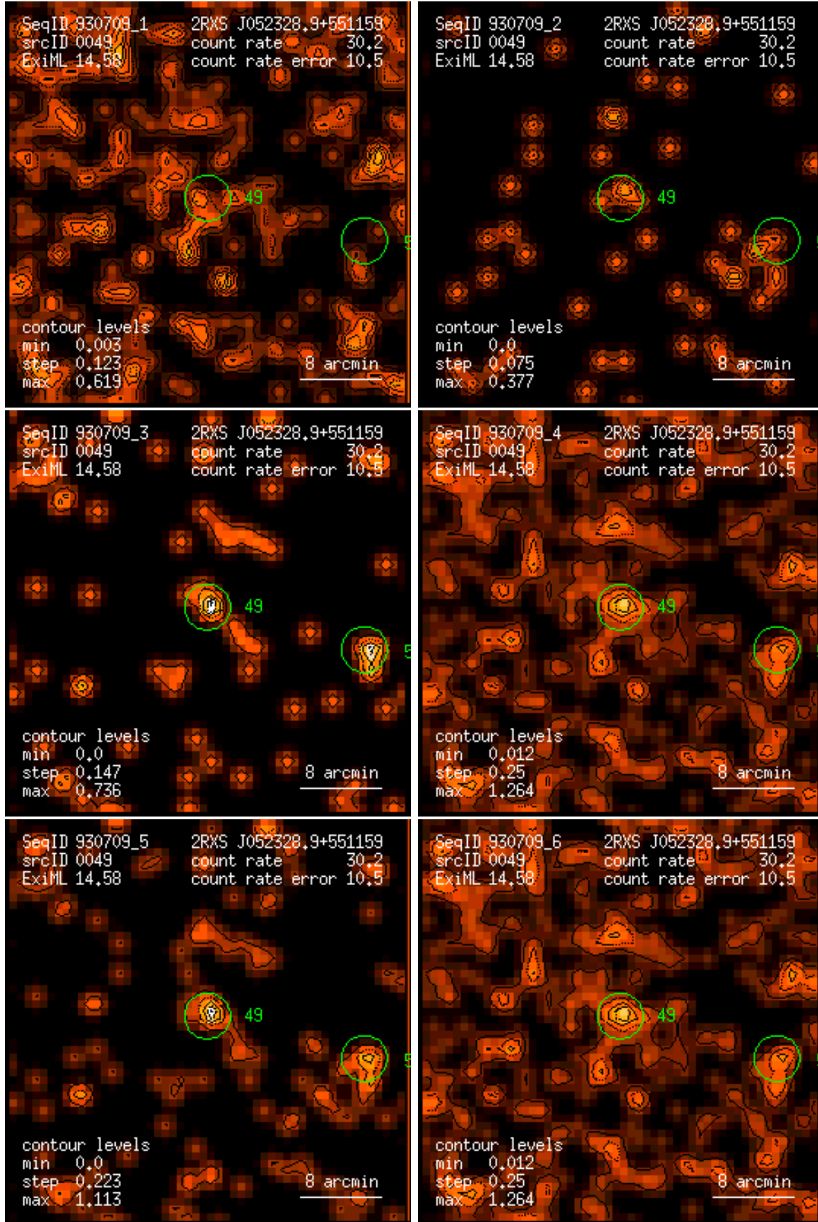
Figure 49: RASS 930709: detection 0049: band rate images, Gaussian filter: (1) PSPC channels 11 – 41, (2) 52 – 90, (3) 91 – 201, (4) 11 – 235, (5) 52 – 201, (6) 11 – 201. Broad band rates in counts/ks. Band rate contour levels in counts/ks/arcmin 2 .
