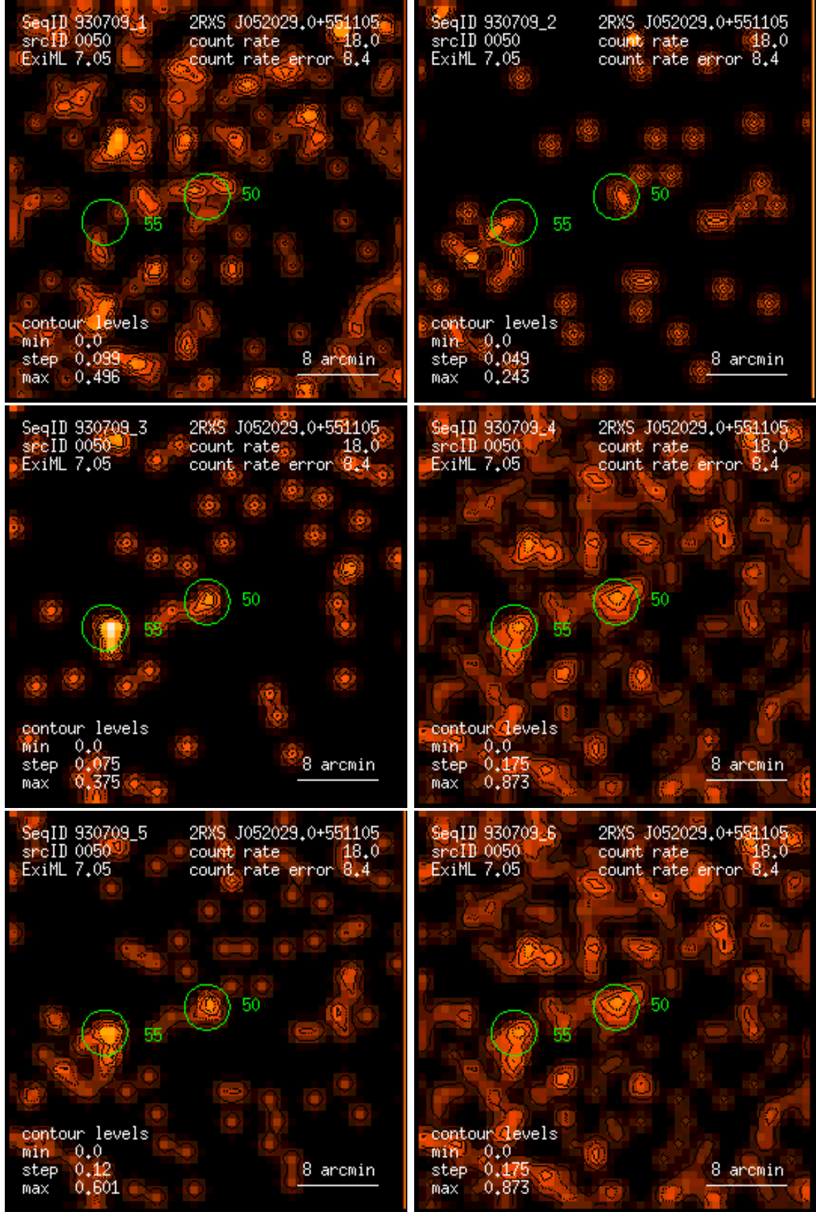
Figure 50: RASS 930709: detection 0050: band rate images, Gaussian filter: (1) PSPC channels 11 – 41, (2) 52 – 90, (3) 91 – 201, (4) 11 – 235, (5) 52 – 201, (6) 11 – 201. Broad band rates in counts/ks. Band rate contour levels in counts/ks/arcmin 2 .
