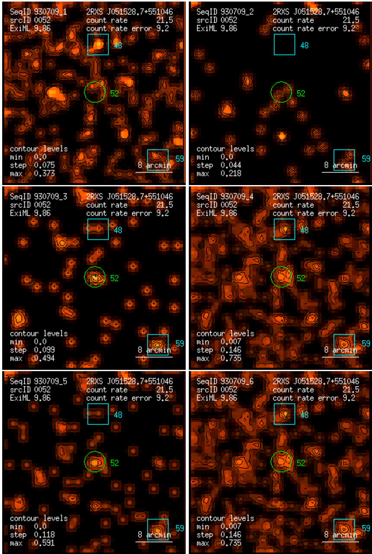
Figure 52: RASS 930709: detection 0052: band rate images, Gaussian filter: (1) PSPC channels 11 – 41, (2) 52 – 90, (3) 91 – 201, (4) 11 – 235, (5) 52 – 201, (6) 11 – 201. Broad band rates in counts/ks. Band rate contour levels in counts/ks/arcmin 2 .
