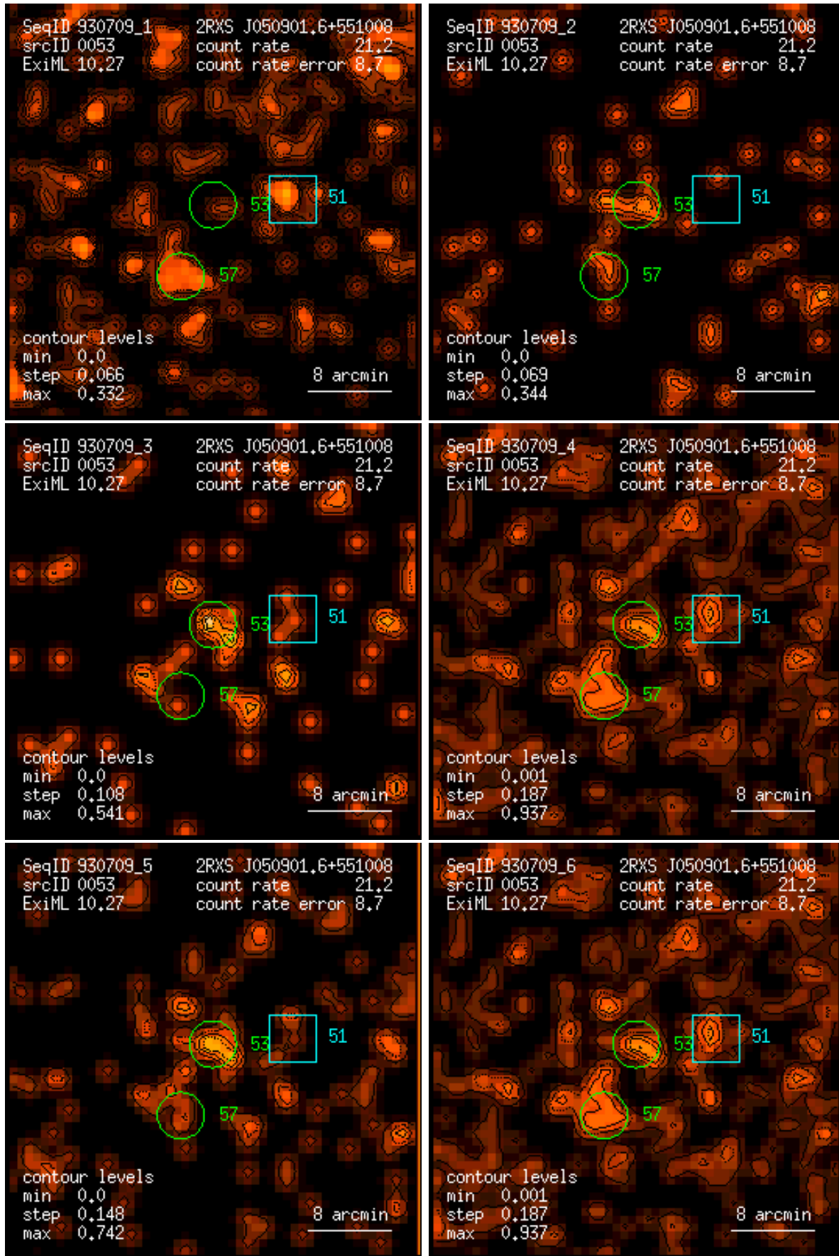
Figure 53: RASS 930709: detection 0053: band rate images, Gaussian filter: (1) PSPC channels 11 – 41, (2) 52 – 90, (3) 91 – 201, (4) 11 – 235, (5) 52 – 201, (6) 11 – 201. Broad band rates in counts/ks. Band rate contour levels in counts/ks/arcmin 2 .
