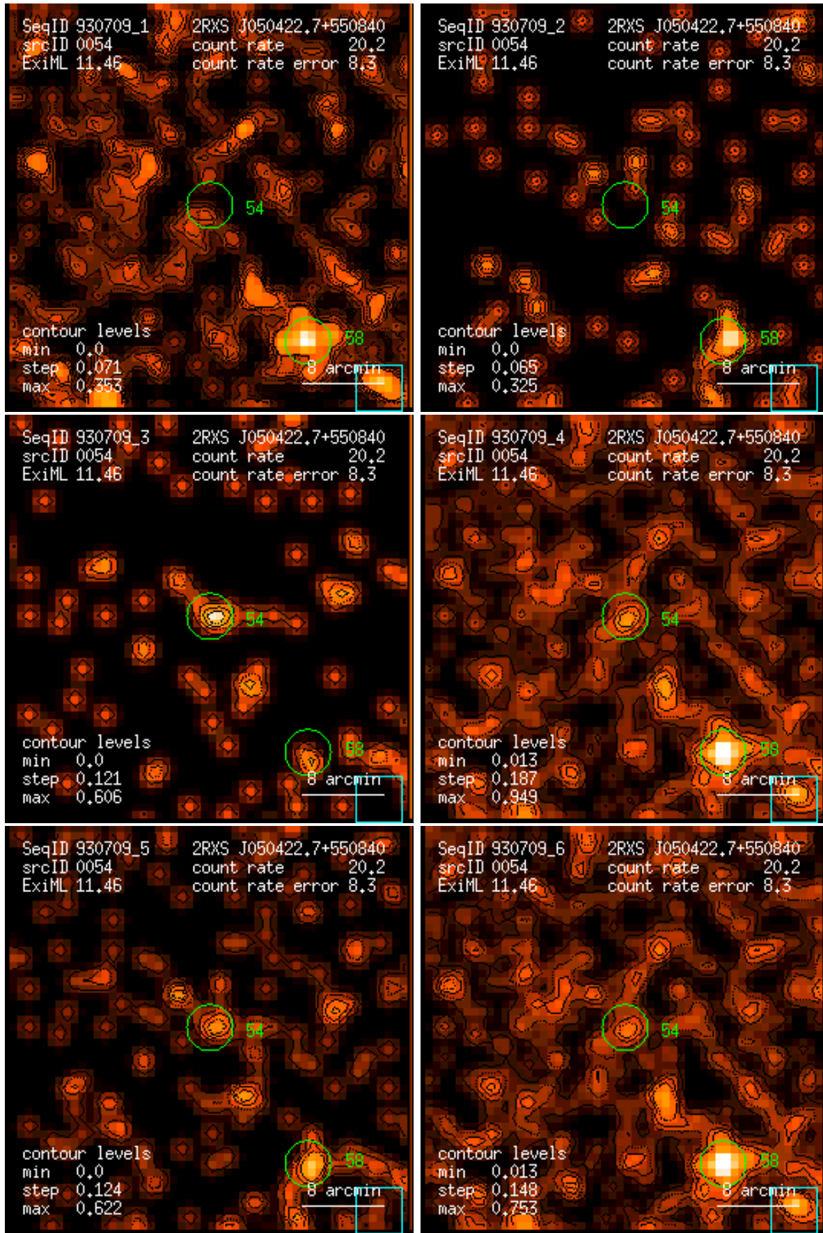
Figure 54: RASS 930709: detection 0054: band rate images, Gaussian filter: (1) PSPC channels 11 – 41, (2) 52 – 90, (3) 91 – 201, (4) 11 – 235, (5) 52 – 201, (6) 11 – 201. Broad band rates in counts/ks. Band rate contour levels in counts/ks/arcmin 2 .
