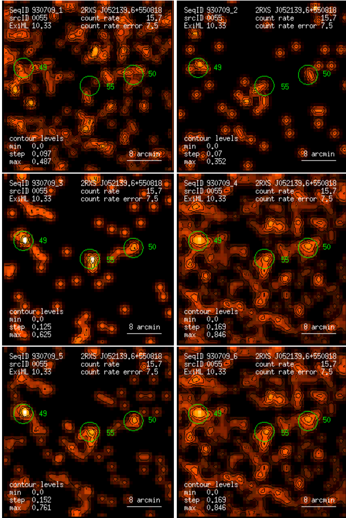
Figure 55: RASS 930709: detection 0055: band rate images, Gaussian filter: (1) PSPC channels 11 – 41, (2) 52 – 90, (3) 91 – 201, (4) 11 – 235, (5) 52 – 201, (6) 11 – 201. Broad band rates in counts/ks. Band rate contour levels in counts/ks/arcmin 2 .
