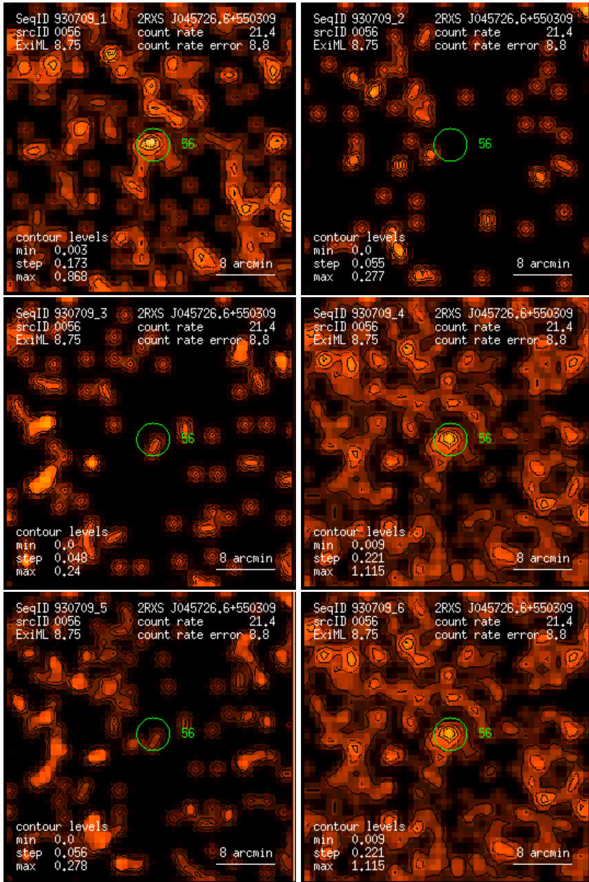
Figure 56: RASS 930709: detection 0056: band rate images, Gaussian filter: (1) PSPC channels 11 – 41, (2) 52 – 90, (3) 91 – 201, (4) 11 – 235, (5) 52 – 201, (6) 11 – 201. Broad band rates in counts/ks. Band rate contour levels in counts/ks/arcmin 2 .
