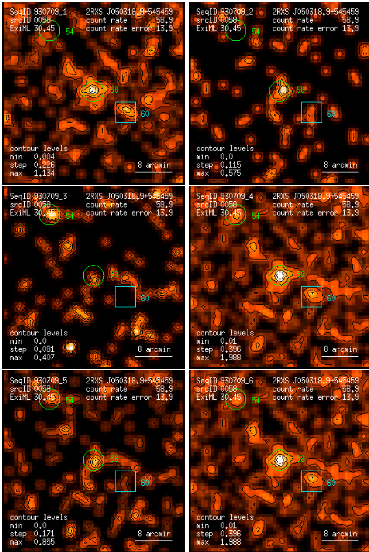
Figure 58: RASS 930709: detection 0058: band rate images, Gaussian filter: (1) PSPC channels 11 – 41, (2) 52 – 90, (3) 91 – 201, (4) 11 – 235, (5) 52 – 201, (6) 11 – 201. Broad band rates in counts/ks. Band rate contour levels in counts/ks/arcmin 2 .
