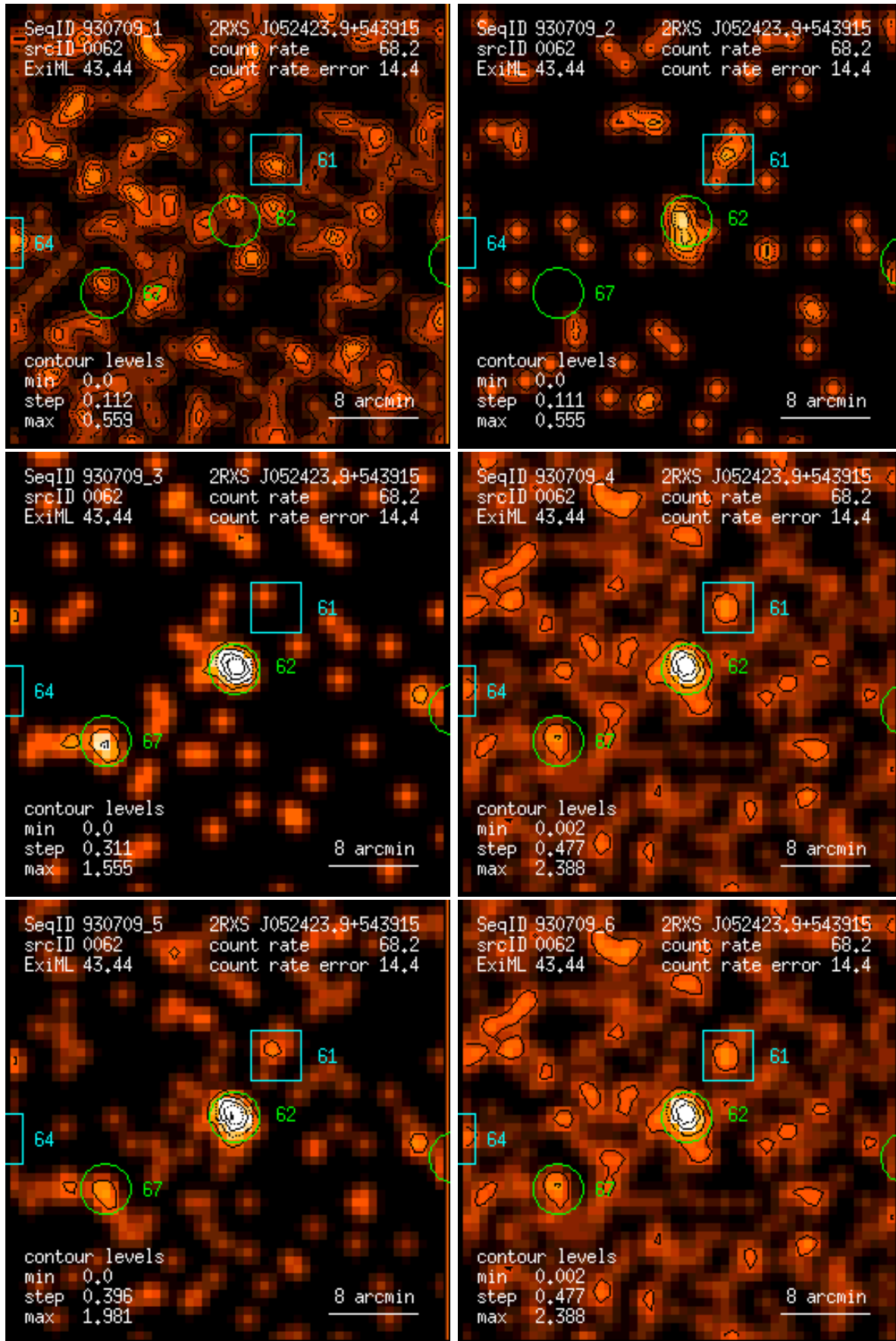
Figure 62: RASS 930709: detection 0062: band rate images, Gaussian filter: (1) PSPC channels 11 – 41, (2) 52 – 90, (3) 91 – 201, (4) 11 – 235, (5) 52 – 201, (6) 11 – 201. Broad band rates in counts/ks. Band rate contour levels in counts/ks/arcmin 2 .
