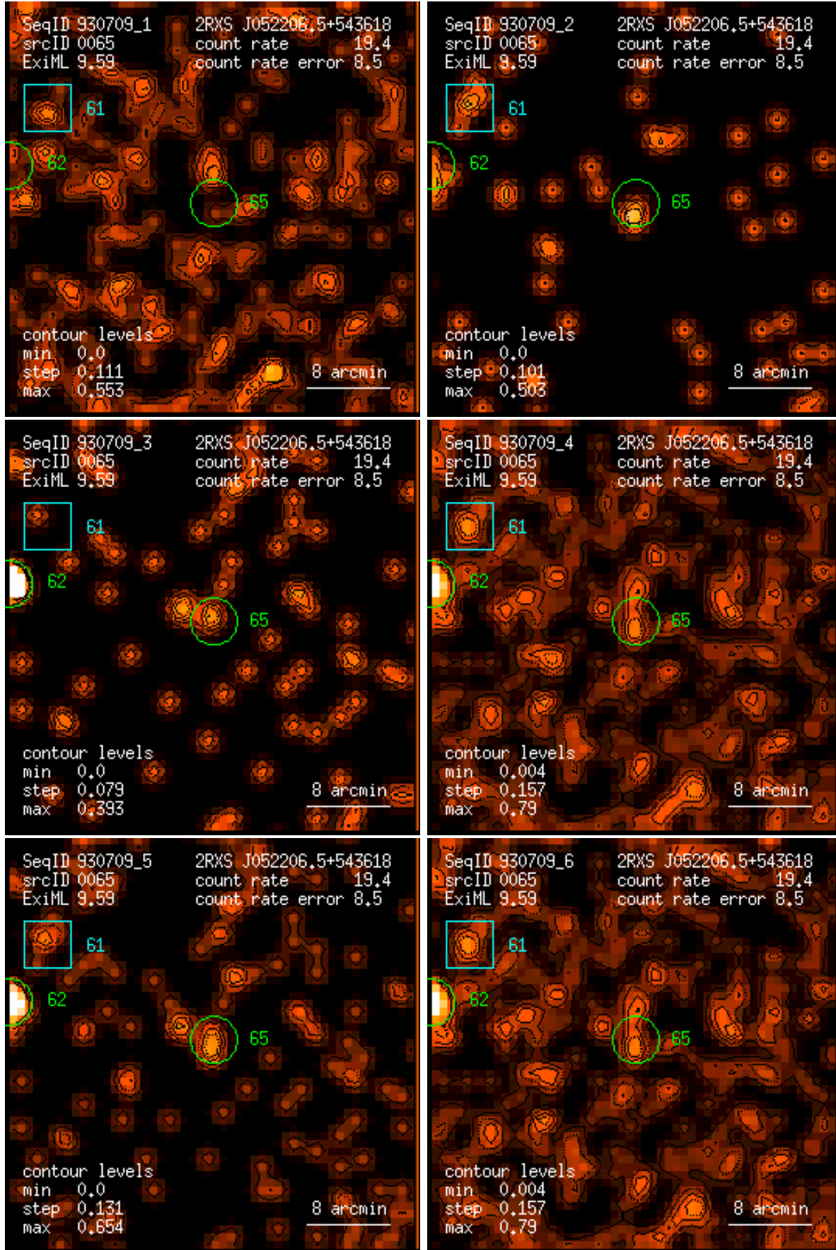
Figure 65: RASS 930709: detection 0065: band rate images, Gaussian filter: (1) PSPC channels 11 – 41, (2) 52 – 90, (3) 91 – 201, (4) 11 – 235, (5) 52 – 201, (6) 11 – 201. Broad band rates in counts/ks. Band rate contour levels in counts/ks/arcmin 2 .
