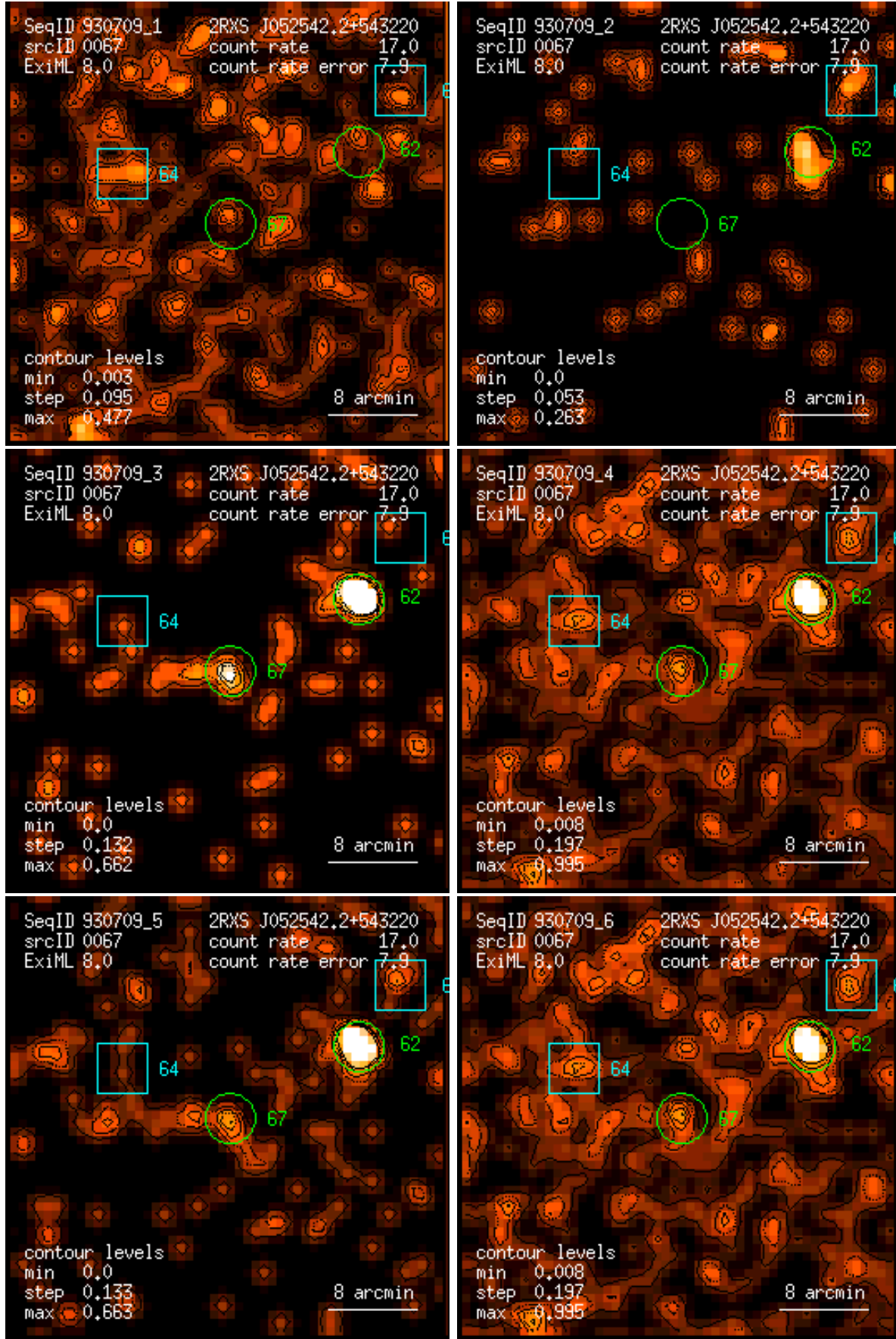
Figure 67: RASS 930709: detection 0067: band rate images, Gaussian filter: (1) PSPC channels 11 – 41, (2) 52 – 90, (3) 91 – 201, (4) 11 – 235, (5) 52 – 201, (6) 11 – 201. Broad band rates in counts/ks. Band rate contour levels in counts/ks/arcmin 2 .
