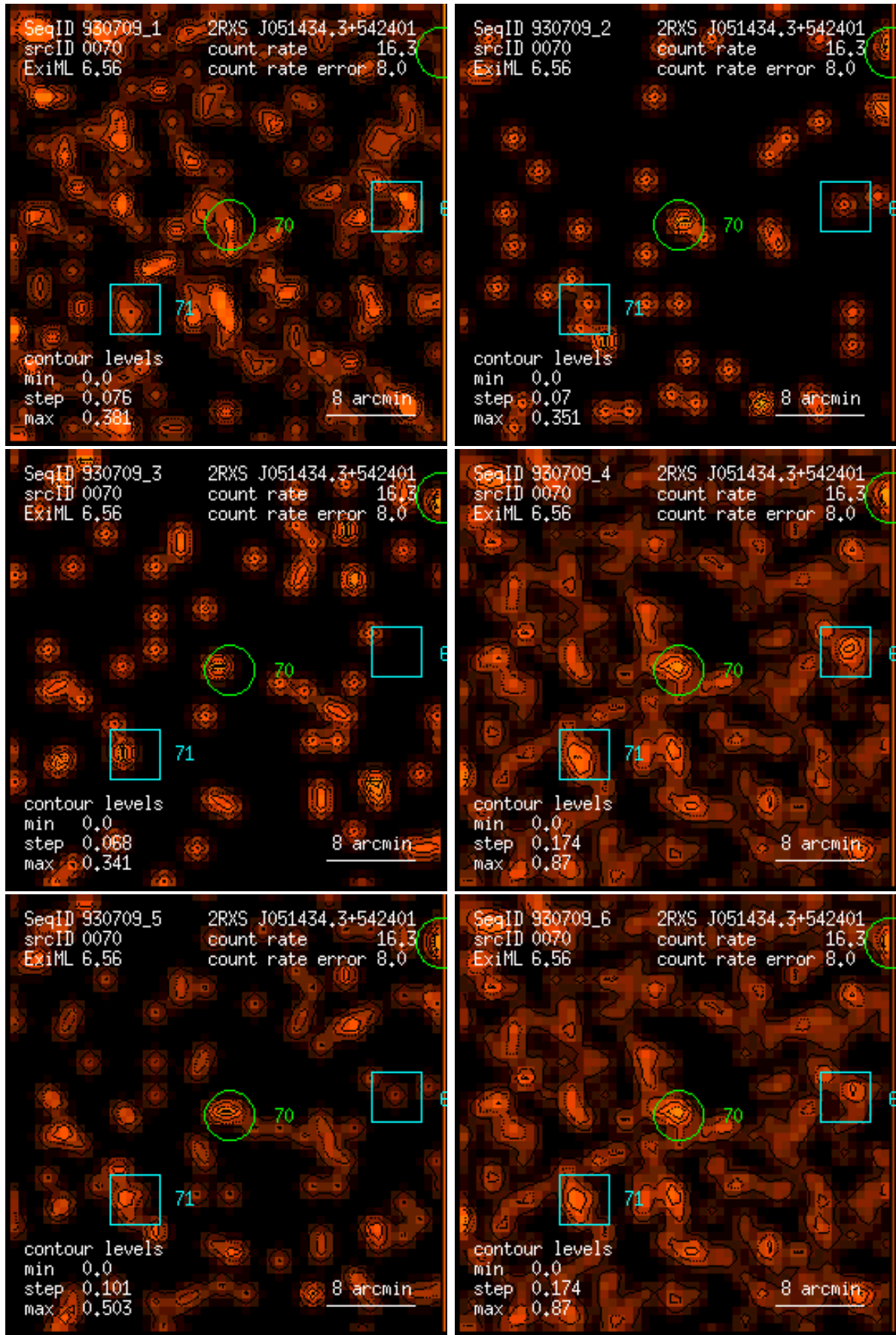
Figure 70: RASS 930709: detection 0070: band rate images, Gaussian filter: (1) PSPC channels 11 – 41, (2) 52 – 90, (3) 91 – 201, (4) 11 – 235, (5) 52 – 201, (6) 11 – 201. Broad band rates in counts/ks. Band rate contour levels in counts/ks/arcmin 2 .
