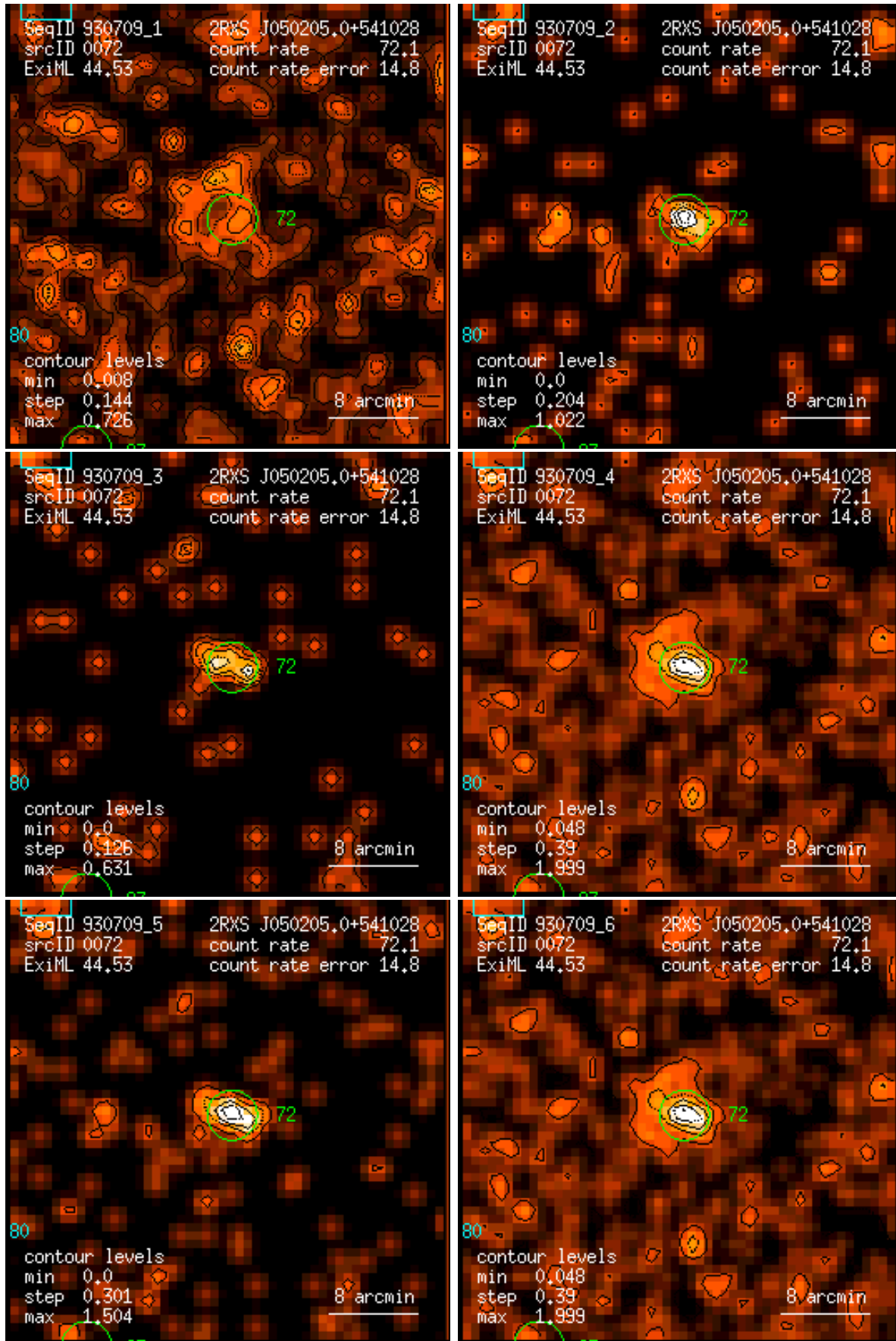
Figure 72: RASS 930709: detection 0072: band rate images, Gaussian filter: (1) PSPC channels 11 – 41, (2) 52 – 90, (3) 91 – 201, (4) 11 – 235, (5) 52 – 201, (6) 11 – 201. Broad band rates in counts/ks. Band rate contour levels in counts/ks/arcmin 2 .
