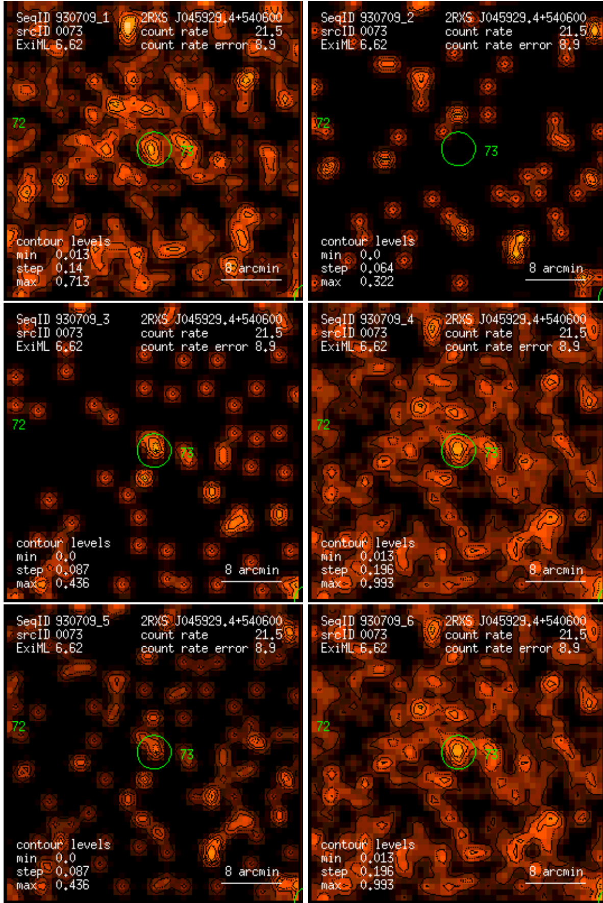
Figure 73: RASS 930709: detection 0073: band rate images, Gaussian filter: (1) PSPC channels 11 – 41, (2) 52 – 90, (3) 91 – 201, (4) 11 – 235, (5) 52 – 201, (6) 11 – 201. Broad band rates in counts/ks. Band rate contour levels in counts/ks/arcmin 2 .
