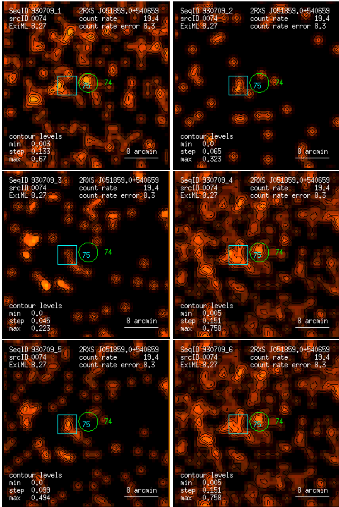
Figure 74: RASS 930709: detection 0074: band rate images, Gaussian filter: (1) PSPC channels 11 – 41, (2) 52 – 90, (3) 91 – 201, (4) 11 – 235, (5) 52 – 201, (6) 11 – 201. Broad band rates in counts/ks. Band rate contour levels in counts/ks/arcmin 2 .
