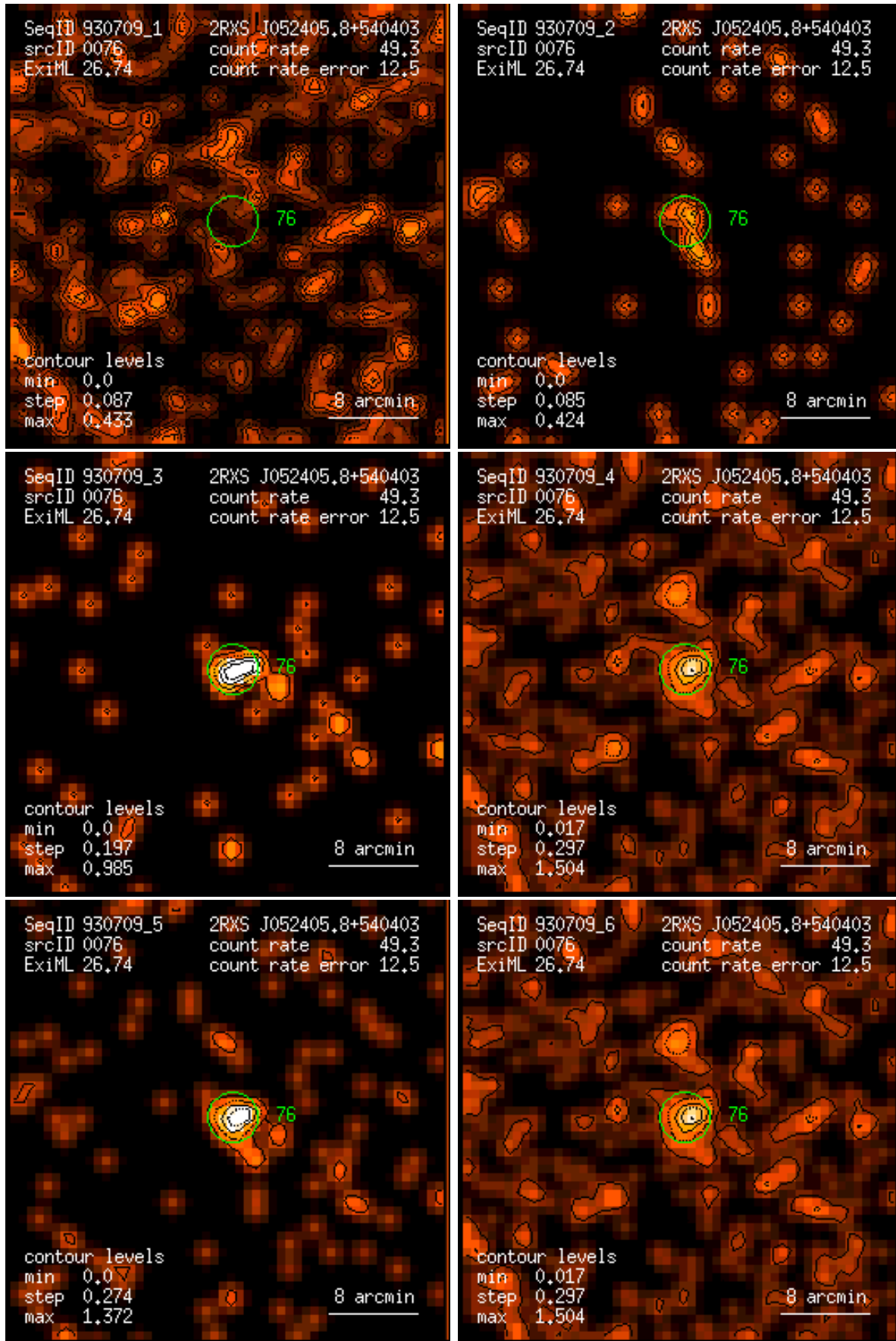
Figure 76: RASS 930709: detection 0076: band rate images, Gaussian filter: (1) PSPC channels 11 – 41, (2) 52 – 90, (3) 91 – 201, (4) 11 – 235, (5) 52 – 201, (6) 11 – 201. Broad band rates in counts/ks. Band rate contour levels in counts/ks/arcmin 2 .
