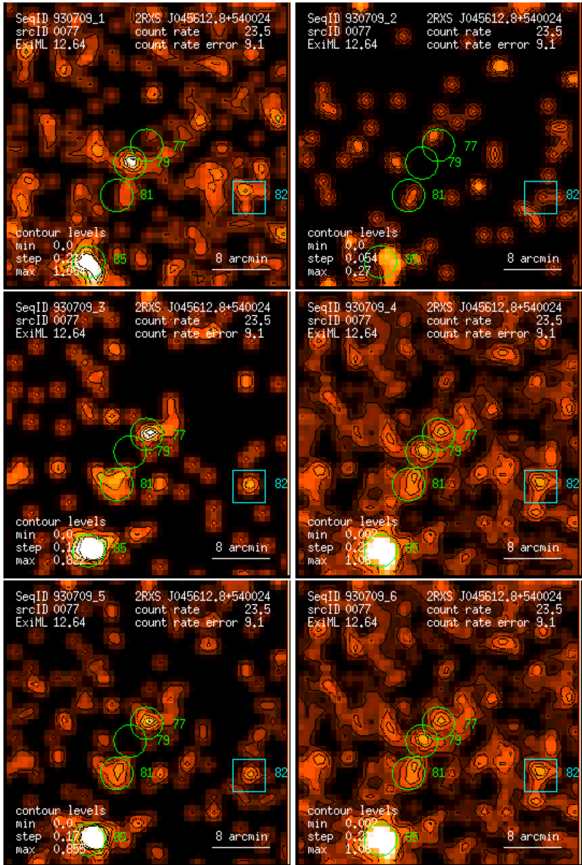
Figure 77: RASS 930709: detection 0077: band rate images, Gaussian filter: (1) PSPC channels 11 – 41, (2) 52 – 90, (3) 91 – 201, (4) 11 – 235, (5) 52 – 201, (6) 11 – 201. Broad band rates in counts/ks. Band rate contour levels in counts/ks/arcmin 2 .
