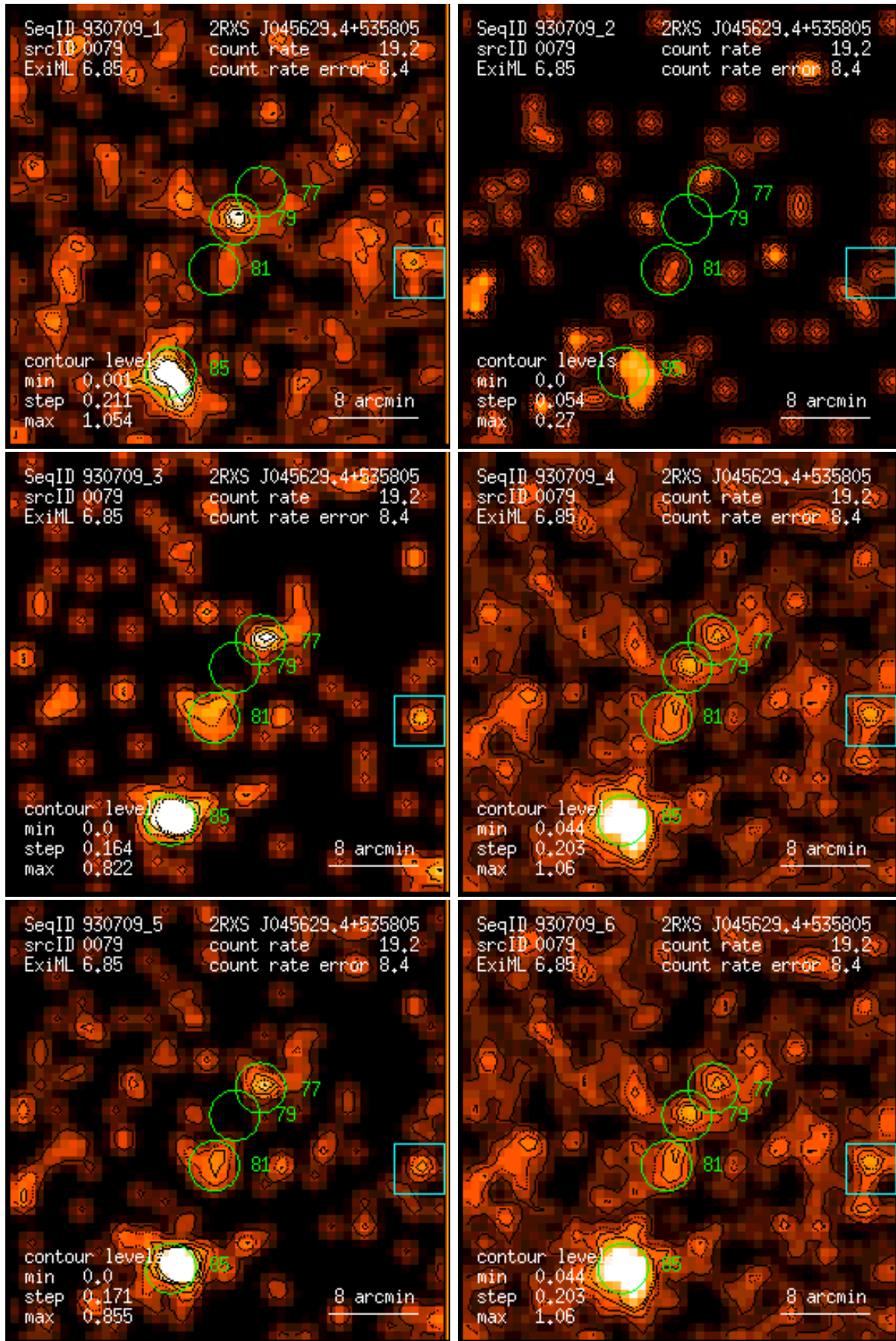
Figure 79: RASS 930709: detection 0079: band rate images, Gaussian filter: (1) PSPC channels 11 – 41, (2) 52 – 90, (3) 91 – 201, (4) 11 – 235, (5) 52 – 201, (6) 11 – 201. Broad band rates in counts/ks. Band rate contour levels in counts/ks/arcmin 2 .
