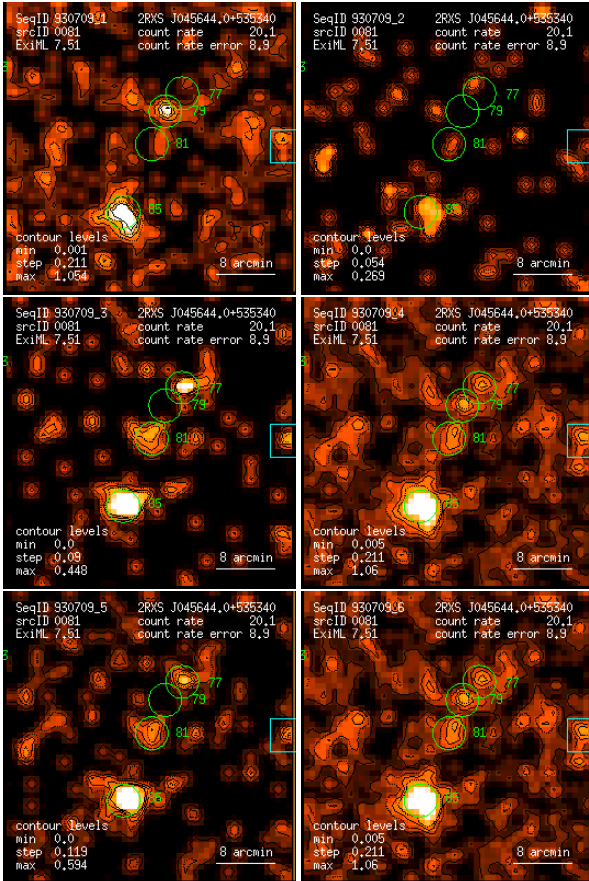
Figure 81: RASS 930709: detection 0081: band rate images, Gaussian filter: (1) PSPC channels 11 – 41, (2) 52 – 90, (3) 91 – 201, (4) 11 – 235, (5) 52 – 201, (6) 11 – 201. Broad band rates in counts/ks. Band rate contour levels in counts/ks/arcmin 2 .
