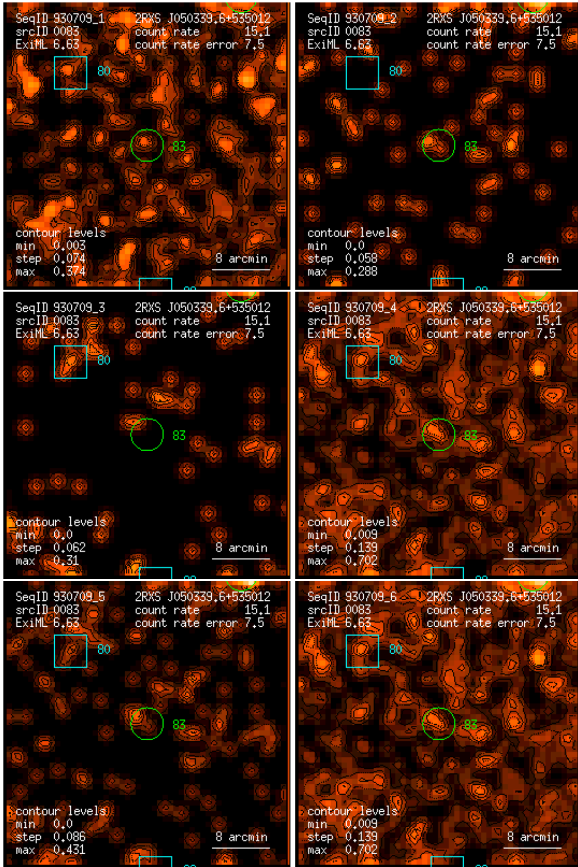
Figure 83: RASS 930709: detection 0083: band rate images, Gaussian filter: (1) PSPC channels 11 – 41, (2) 52 – 90, (3) 91 – 201, (4) 11 – 235, (5) 52 – 201, (6) 11 – 201. Broad band rates in counts/ks. Band rate contour levels in counts/ks/arcmin 2 .
