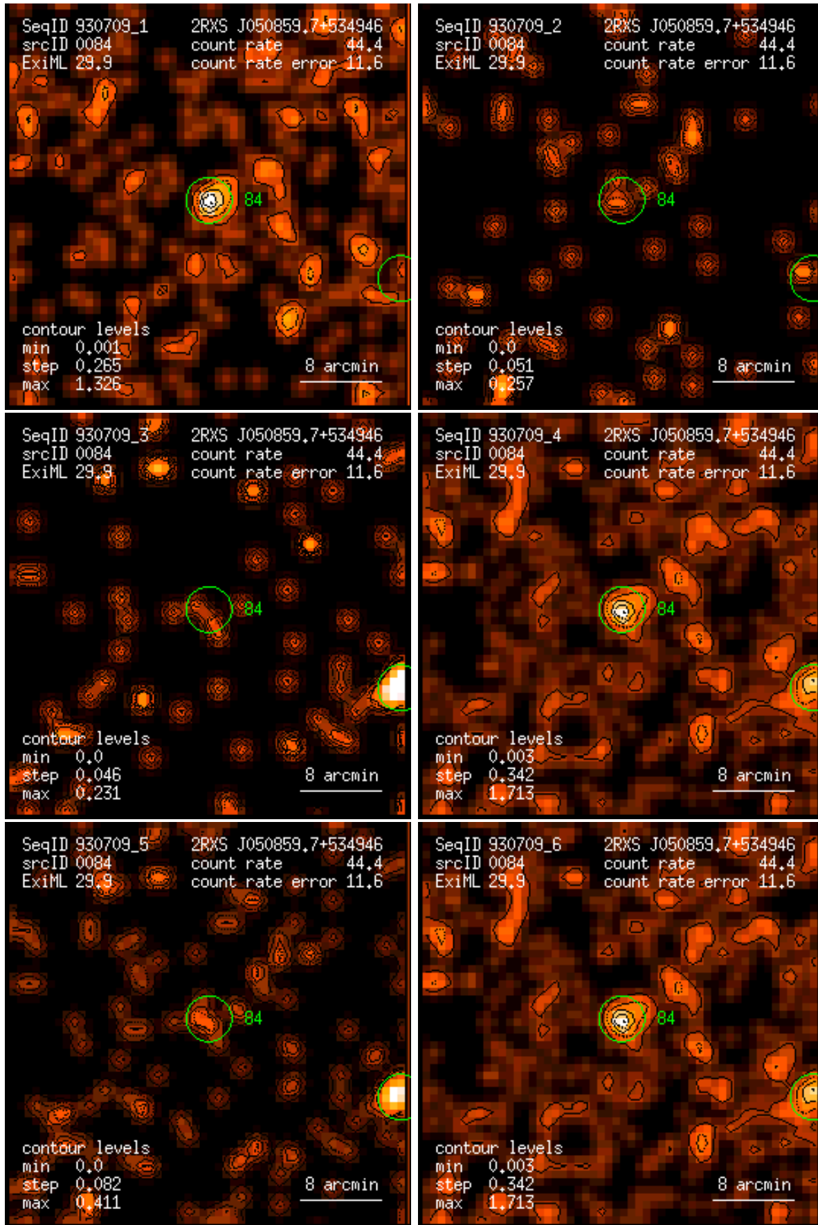
Figure 84: RASS 930709: detection 0084: band rate images, Gaussian filter: (1) PSPC channels 11 – 41, (2) 52 – 90, (3) 91 – 201, (4) 11 – 235, (5) 52 – 201, (6) 11 – 201. Broad band rates in counts/ks. Band rate contour levels in counts/ks/arcmin 2 .
