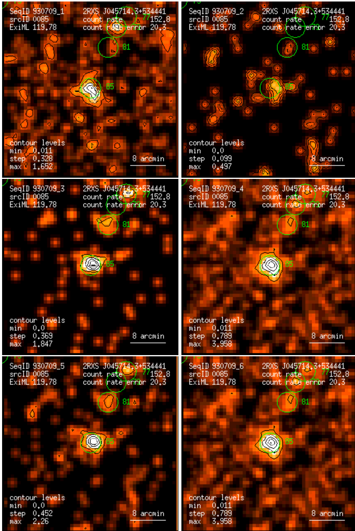
Figure 85: RASS 930709: detection 0085: band rate images, Gaussian filter: (1) PSPC channels 11 – 41, (2) 52 – 90, (3) 91 – 201, (4) 11 – 235, (5) 52 – 201, (6) 11 – 201. Broad band rates in counts/ks. Band rate contour levels in counts/ks/arcmin 2 .
