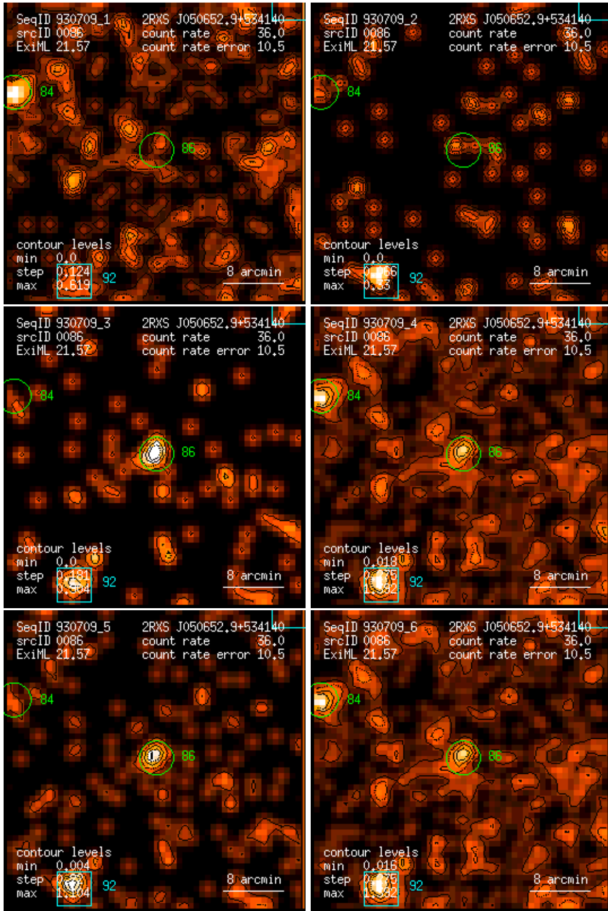
Figure 86: RASS 930709: detection 0086: band rate images, Gaussian filter: (1) PSPC channels 11 – 41, (2) 52 – 90, (3) 91 – 201, (4) 11 – 235, (5) 52 – 201, (6) 11 – 201. Broad band rates in counts/ks. Band rate contour levels in counts/ks/arcmin 2 .
